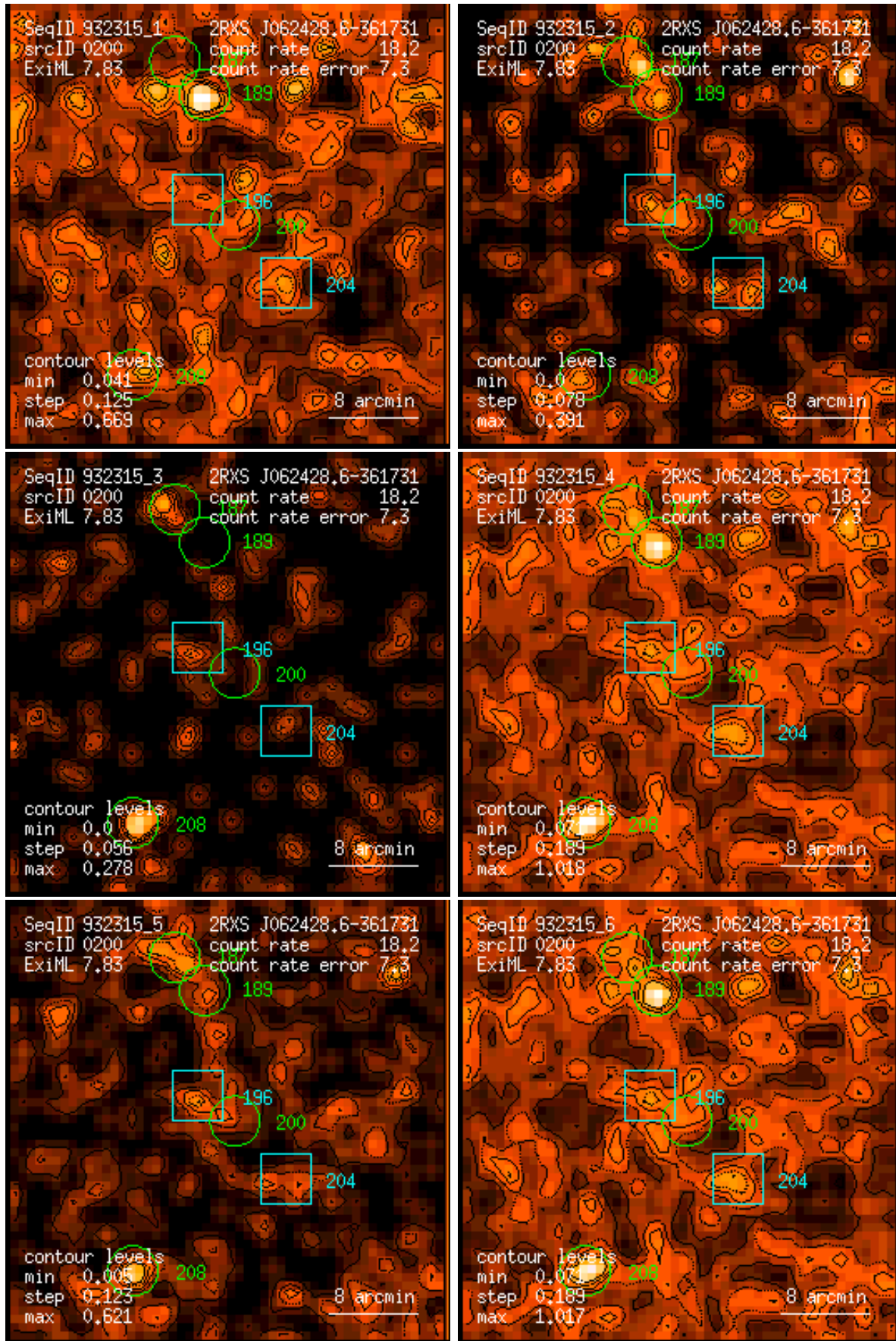
Figure 200: RASS 932315: detection 0200: band rate images, Gaussian filter: (1) PSPC channels 11 – 41, (2) 52 – 90, (3) 91 – 201, (4) 11 – 235, (5) 52 – 201, (6) 11 – 201. Broad band rates in counts/ks. Band rate contour levels in counts/ks/arcmin 2 .
