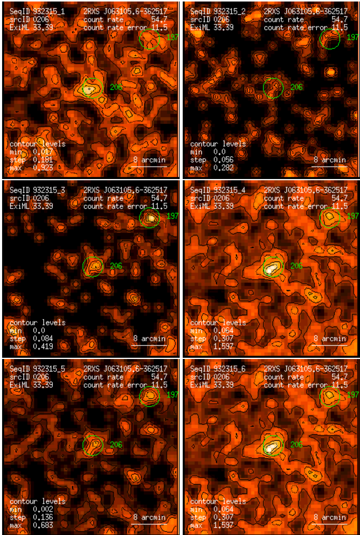
Figure 206: RASS 932315: detection 0206: band rate images, Gaussian filter: (1) PSPC channels 11 – 41, (2) 52 – 90, (3) 91 – 201, (4) 11 – 235, (5) 52 – 201, (6) 11 – 201. Broad band rates in counts/ks. Band rate contour levels in counts/ks/arcmin 2 .
