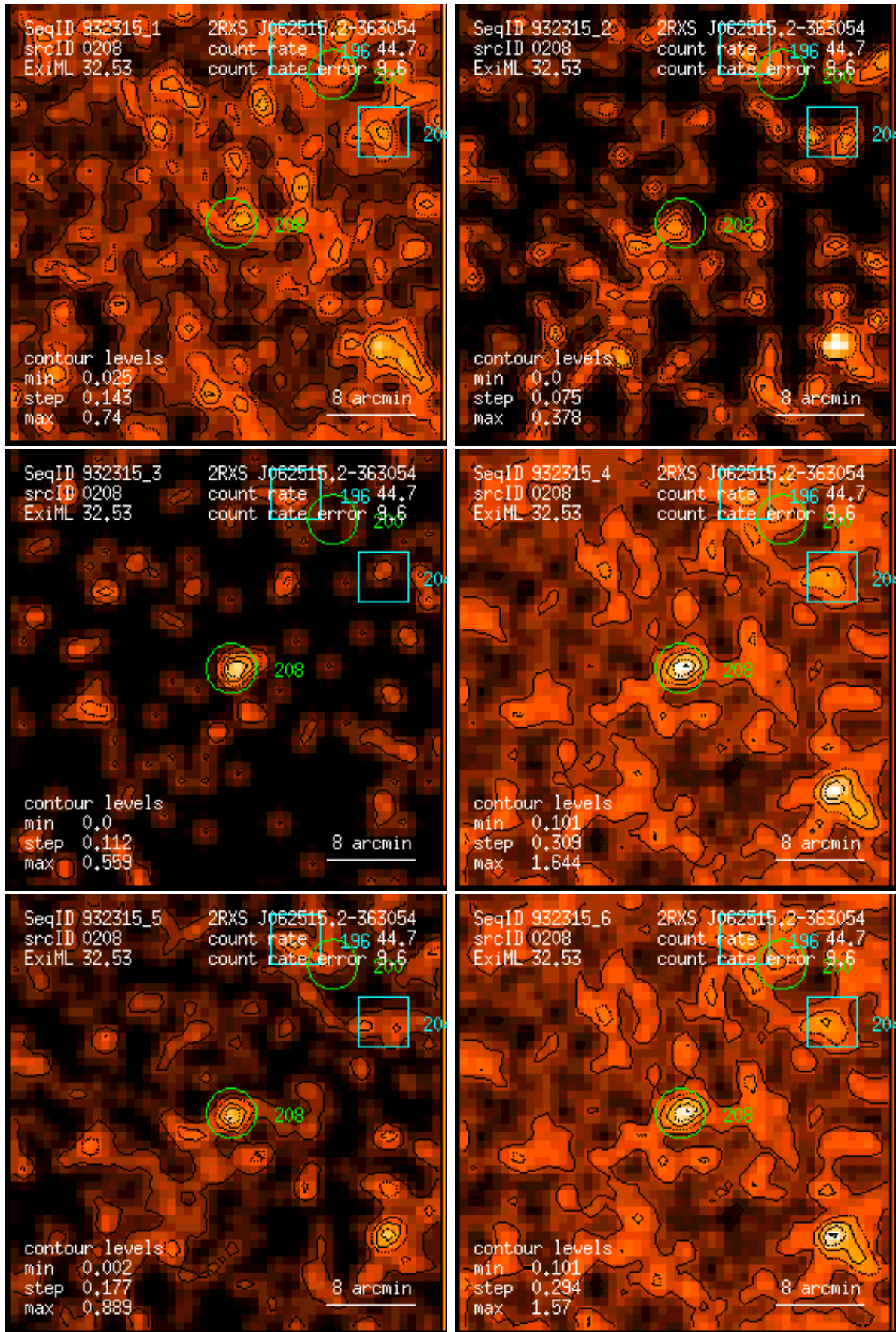
Figure 208: RASS 932315: detection 0208: band rate images, Gaussian filter: (1) PSPC channels 11 – 41, (2) 52 – 90, (3) 91 – 201, (4) 11 – 235, (5) 52 – 201, (6) 11 – 201. Broad band rates in counts/ks. Band rate contour levels in counts/ks/arcmin 2 .
