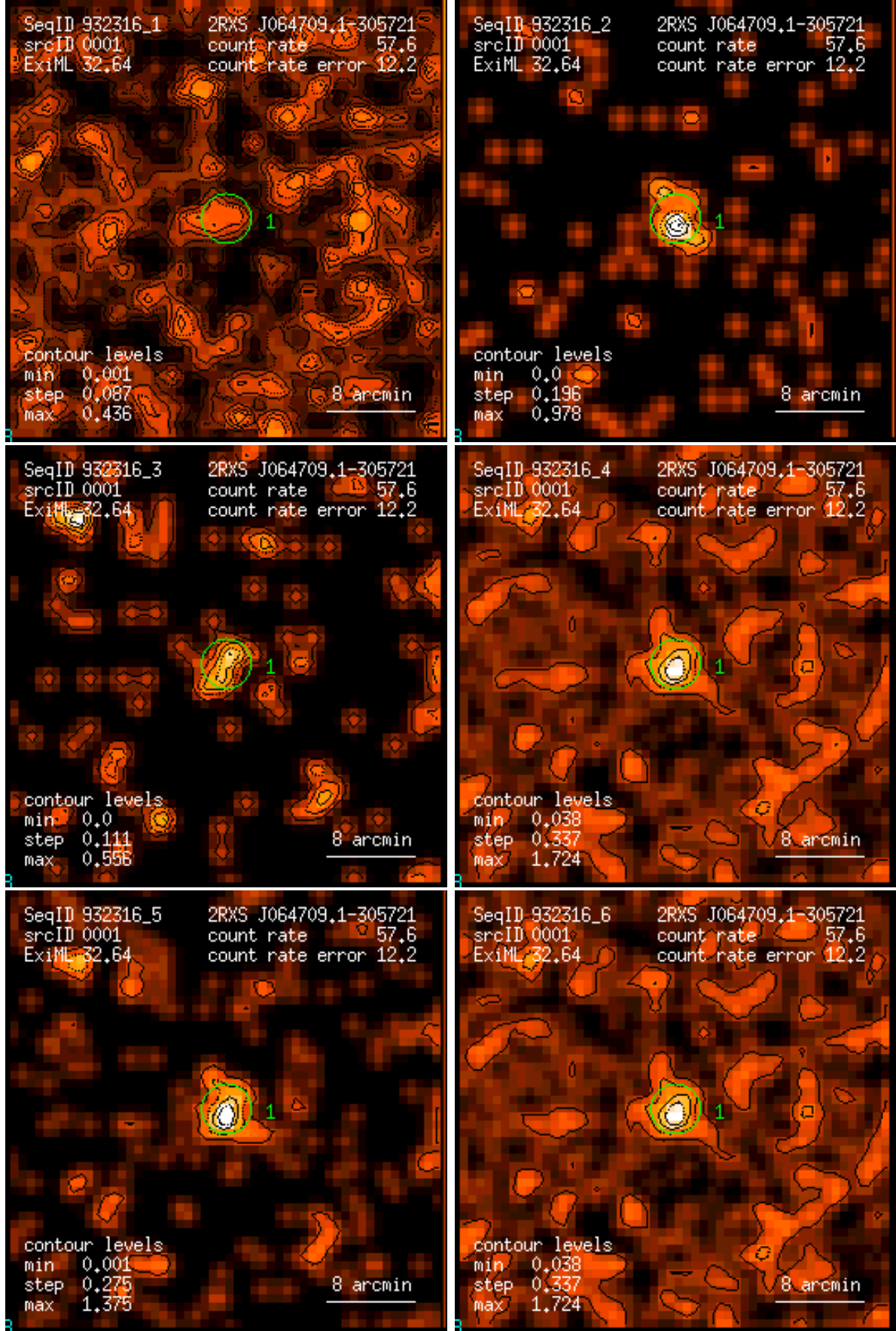
Figure 1: RASS 932316: detection 0001: band rate images, Gaussian filter: (1) PSPC channels 11 – 41, (2) 52 – 90, (3) 91 – 201, (4) 11 – 235, (5) 52 – 201, (6) 11 – 201. Broad band rates in counts/ks. Band rate contour levels in counts/ks/arcmin 2 .
