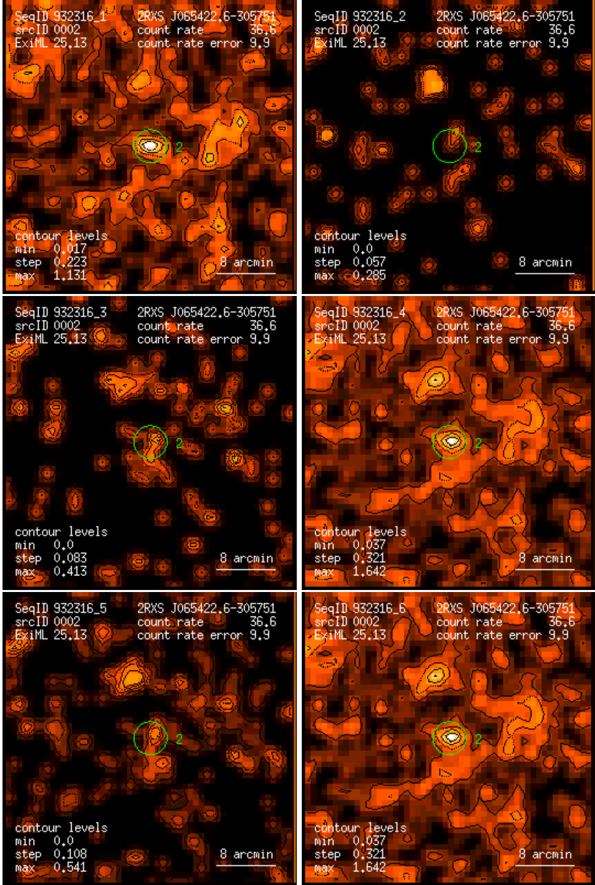
Figure 2: RASS 932316: detection 0002: band rate images, Gaussian filter: (1) PSPC channels 11 – 41, (2) 52 – 90, (3) 91 – 201, (4) 11 – 235, (5) 52 – 201, (6) 11 – 201. Broad band rates in counts/ks. Band rate contour levels in counts/ks/arcmin 2 .
