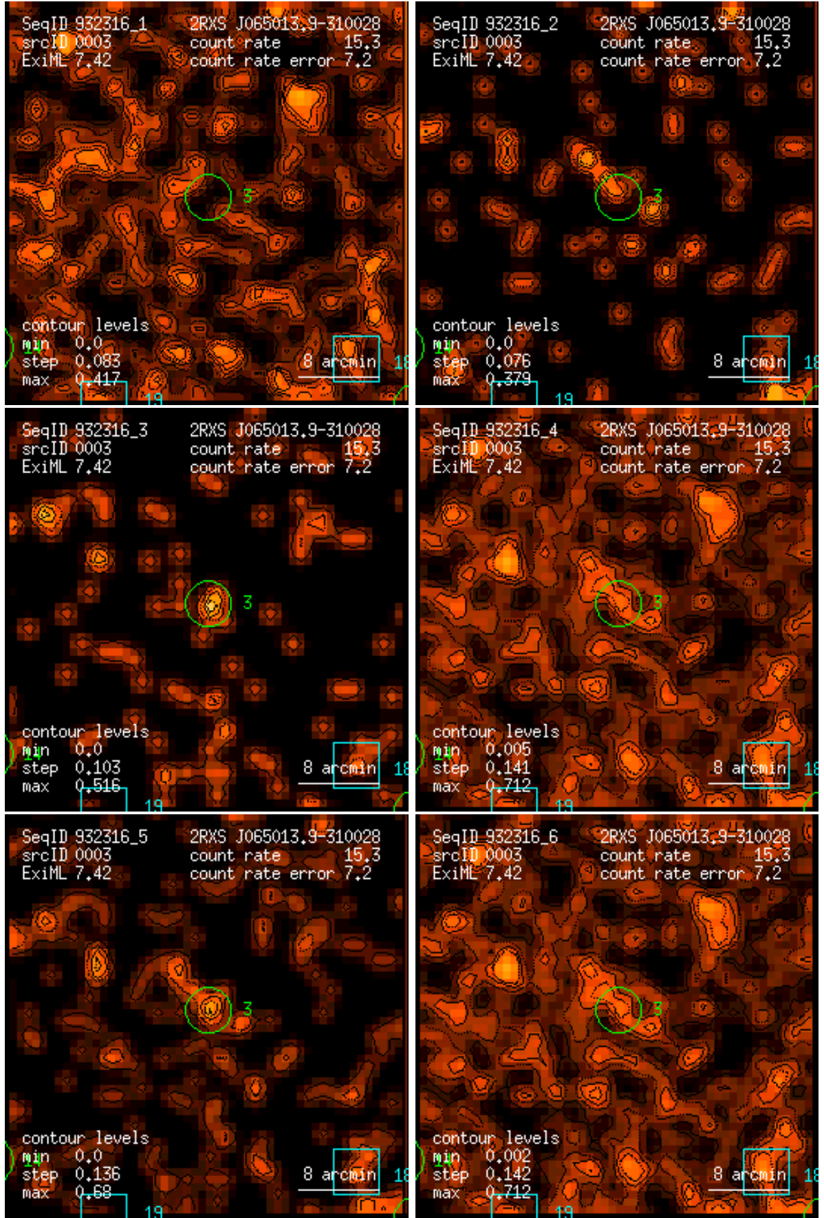
Figure 3: RASS 932316: detection 0003: band rate images, Gaussian filter: (1) PSPC channels 11 – 41, (2) 52 – 90, (3) 91 – 201, (4) 11 – 235, (5) 52 – 201, (6) 11 – 201. Broad band rates in counts/ks. Band rate contour levels in counts/ks/arcmin 2 .
