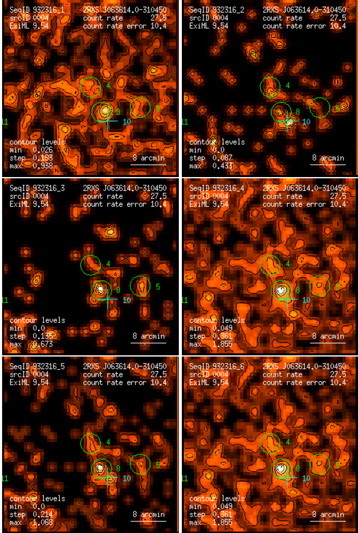
Figure 4: RASS 932316: detection 0004: band rate images, Gaussian filter: (1) PSPC channels 11 – 41, (2) 52 – 90, (3) 91 – 201, (4) 11 – 235, (5) 52 – 201, (6) 11 – 201. Broad band rates in counts/ks. Band rate contour levels in counts/ks/arcmin 2 .
