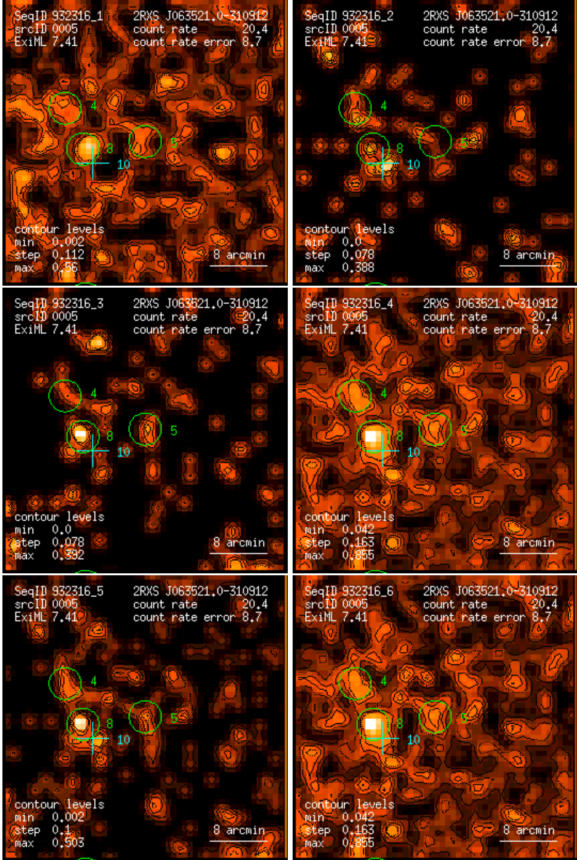
Figure 5: RASS 932316: detection 0005: band rate images, Gaussian filter: (1) PSPC channels 11 – 41, (2) 52 – 90, (3) 91 – 201, (4) 11 – 235, (5) 52 – 201, (6) 11 – 201. Broad band rates in counts/ks. Band rate contour levels in counts/ks/arcmin 2 .
