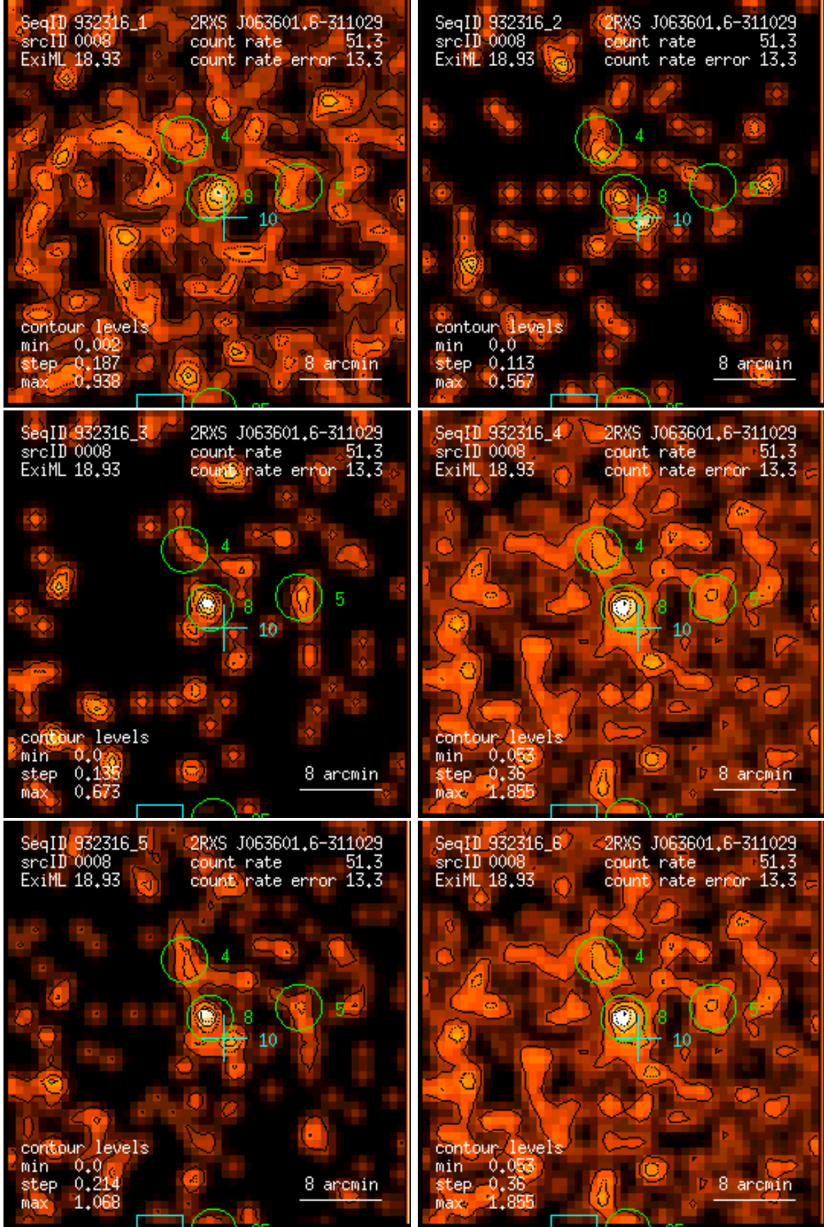
Figure 8: RASS 932316: detection 0008: band rate images, Gaussian filter: (1) PSPC channels 11 – 41, (2) 52 – 90, (3) 91 – 201, (4) 11 – 235, (5) 52 – 201, (6) 11 – 201. Broad band rates in counts/ks. Band rate contour levels in counts/ks/arcmin 2 .
