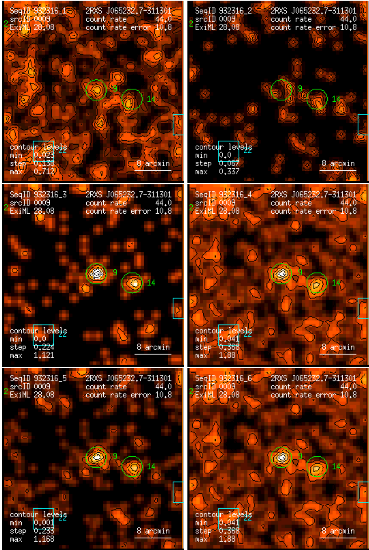
Figure 9: RASS 932316: detection 0009: band rate images, Gaussian filter: (1) PSPC channels 11 – 41, (2) 52 – 90, (3) 91 – 201, (4) 11 – 235, (5) 52 – 201, (6) 11 – 201. Broad band rates in counts/ks. Band rate contour levels in counts/ks/arcmin 2 .
