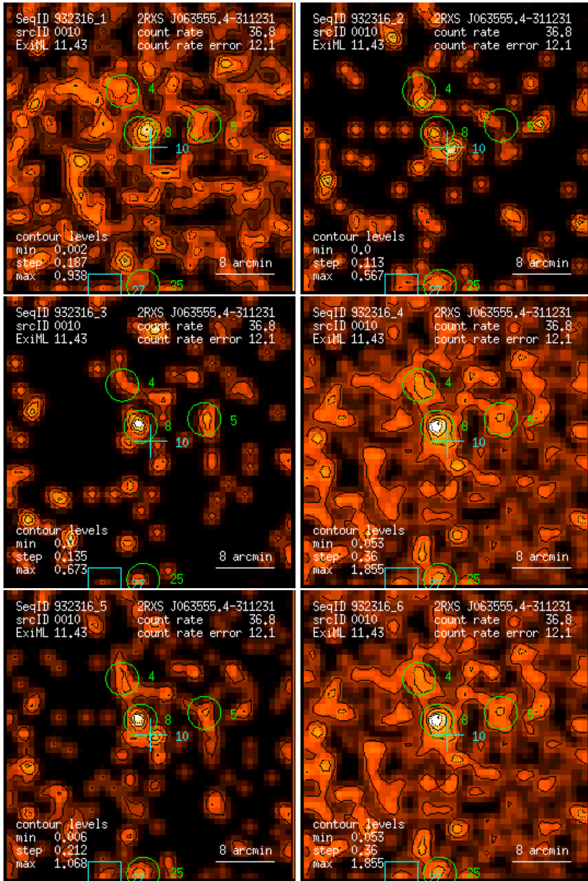
Figure 10: RASS 932316: detection 0010: band rate images, Gaussian filter: (1) PSPC channels 11 – 41, (2) 52 – 90, (3) 91 – 201, (4) 11 – 235, (5) 52 – 201, (6) 11 – 201. Broad band rates in counts/ks. Band rate contour levels in counts/ks/arcmin 2 .
