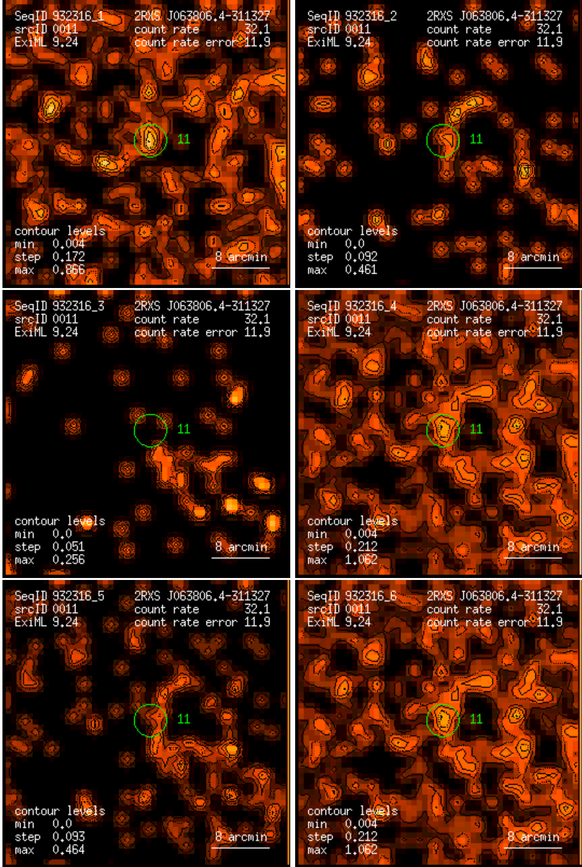
Figure 11: RASS 932316: detection 0011: band rate images, Gaussian filter: (1) PSPC channels 11 – 41, (2) 52 – 90, (3) 91 – 201, (4) 11 – 235, (5) 52 – 201, (6) 11 – 201. Broad band rates in counts/ks. Band rate contour levels in counts/ks/arcmin 2 .
