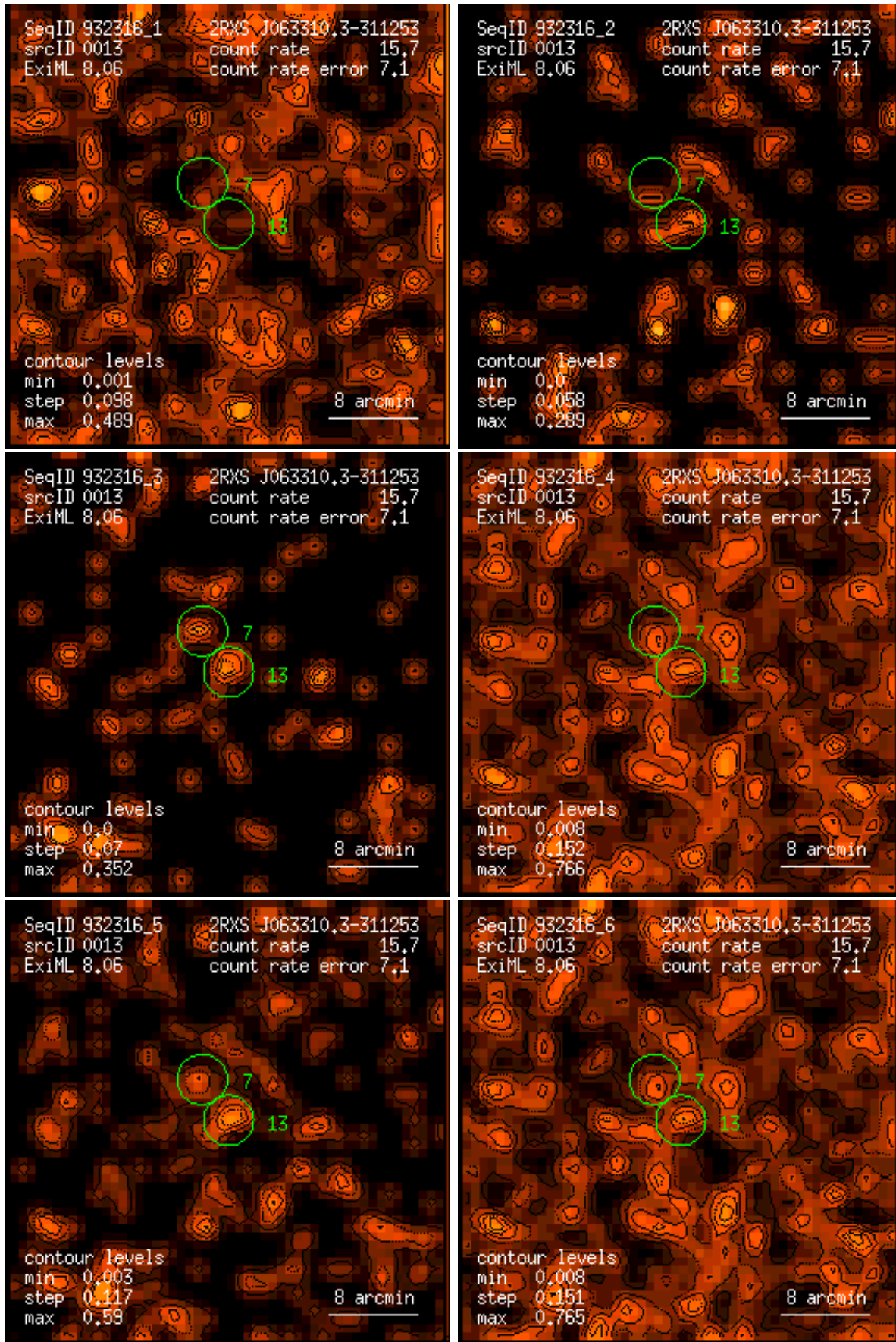
Figure 13: RASS 932316: detection 0013: band rate images, Gaussian filter: (1) PSPC channels 11 – 41, (2) 52 – 90, (3) 91 – 201, (4) 11 – 235, (5) 52 – 201, (6) 11 – 201. Broad band rates in counts/ks. Band rate contour levels in counts/ks/arcmin 2 .
