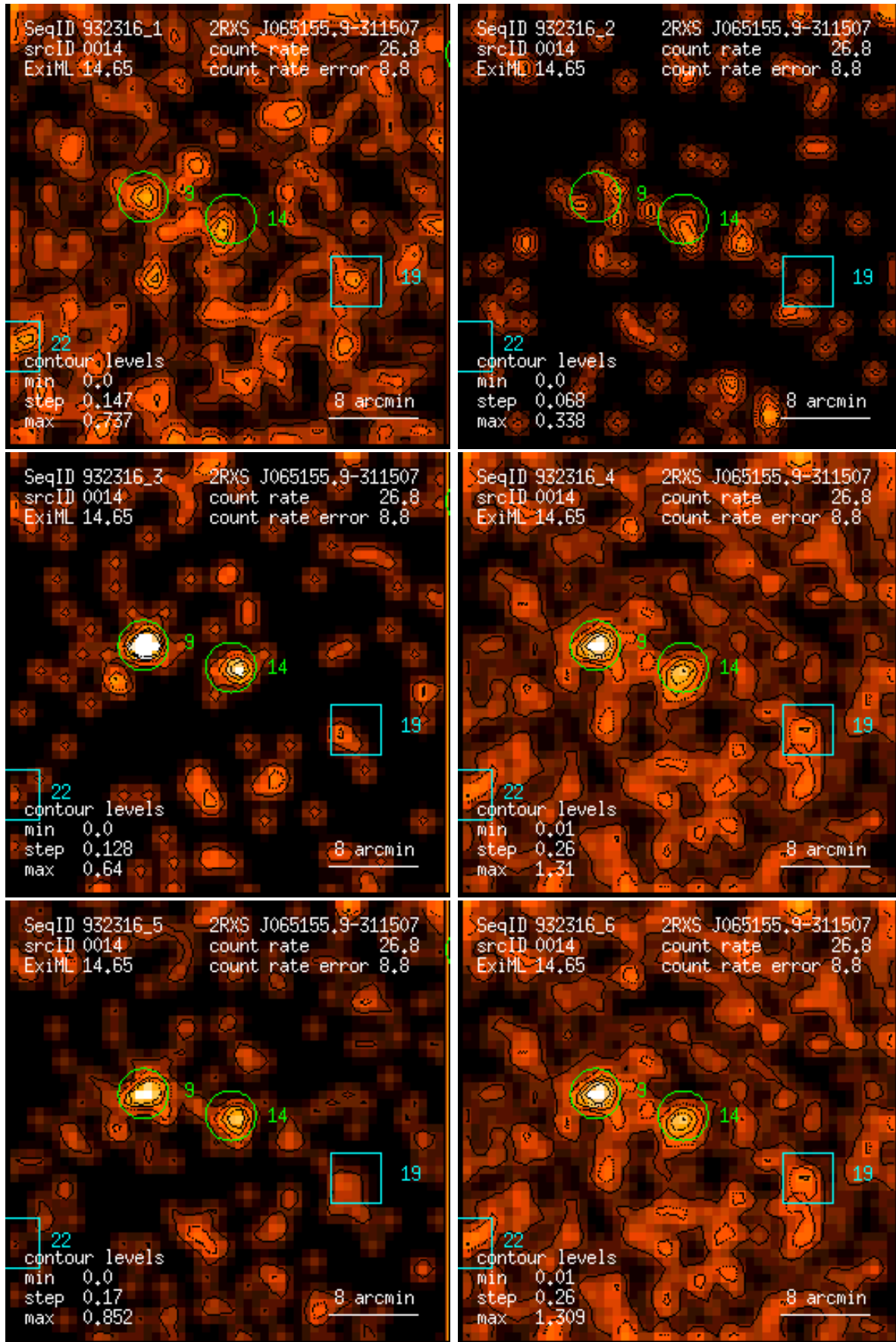
Figure 14: RASS 932316: detection 0014: band rate images, Gaussian filter: (1) PSPC channels 11 – 41, (2) 52 – 90, (3) 91 – 201, (4) 11 – 235, (5) 52 – 201, (6) 11 – 201. Broad band rates in counts/ks. Band rate contour levels in counts/ks/arcmin 2 .
