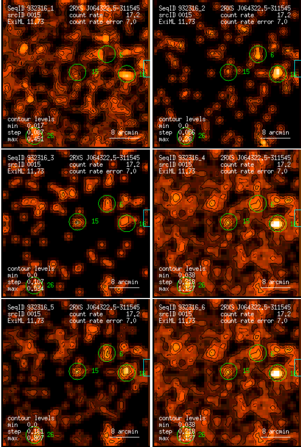
Figure 15: RASS 932316: detection 0015: band rate images, Gaussian filter: (1) PSPC channels 11 – 41, (2) 52 – 90, (3) 91 – 201, (4) 11 – 235, (5) 52 – 201, (6) 11 – 201. Broad band rates in counts/ks. Band rate contour levels in counts/ks/arcmin 2 .
