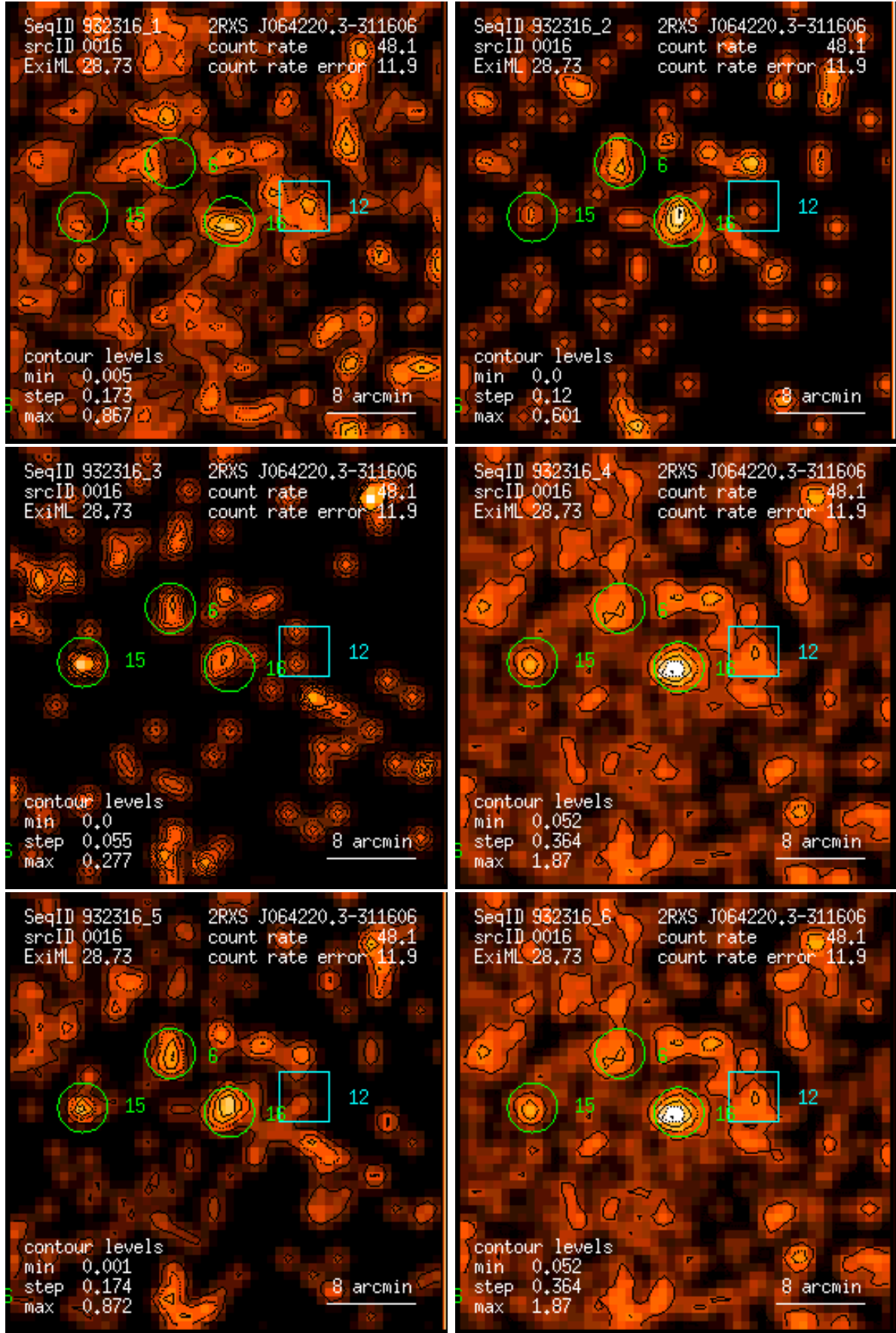
Figure 16: RASS 932316: detection 0016: band rate images, Gaussian filter: (1) PSPC channels 11 – 41, (2) 52 – 90, (3) 91 – 201, (4) 11 – 235, (5) 52 – 201, (6) 11 – 201. Broad band rates in counts/ks. Band rate contour levels in counts/ks/arcmin 2 .
