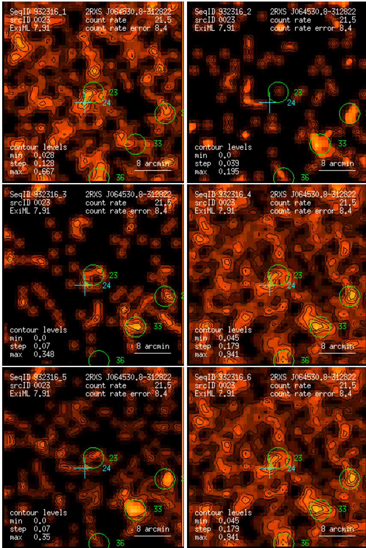
Figure 23: RASS 932316: detection 0023: band rate images, Gaussian filter: (1) PSPC channels 11 – 41, (2) 52 – 90, (3) 91 – 201, (4) 11 – 235, (5) 52 – 201, (6) 11 – 201. Broad band rates in counts/ks. Band rate contour levels in counts/ks/arcmin 2 .
