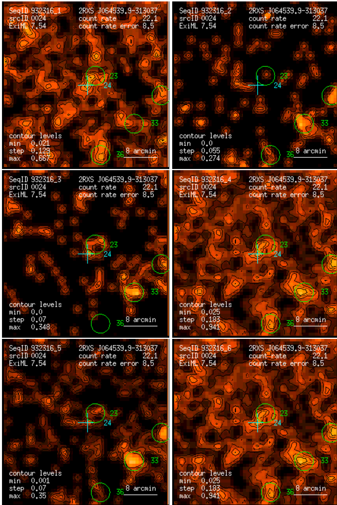
Figure 24: RASS 932316: detection 0024: band rate images, Gaussian filter: (1) PSPC channels 11 – 41, (2) 52 – 90, (3) 91 – 201, (4) 11 – 235, (5) 52 – 201, (6) 11 – 201. Broad band rates in counts/ks. Band rate contour levels in counts/ks/arcmin 2 .
