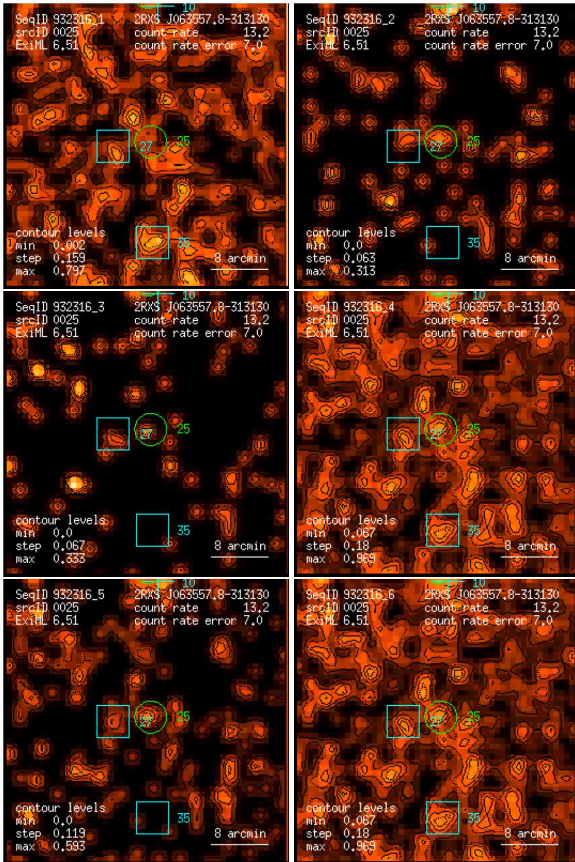
Figure 25: RASS 932316: detection 0025: band rate images, Gaussian filter: (1) PSPC channels 11 – 41, (2) 52 – 90, (3) 91 – 201, (4) 11 – 235, (5) 52 – 201, (6) 11 – 201. Broad band rates in counts/ks. Band rate contour levels in counts/ks/arcmin 2 .
