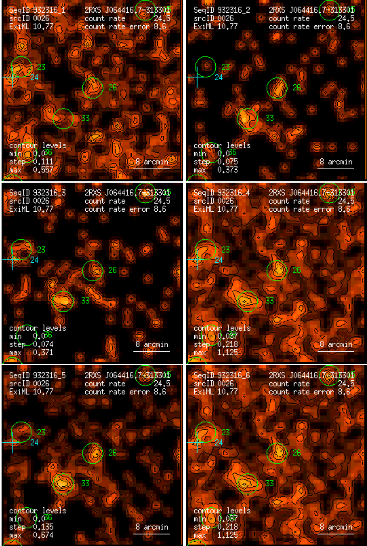
Figure 26: RASS 932316: detection 0026: band rate images, Gaussian filter: (1) PSPC channels 11 – 41, (2) 52 – 90, (3) 91 – 201, (4) 11 – 235, (5) 52 – 201, (6) 11 – 201. Broad band rates in counts/ks. Band rate contour levels in counts/ks/arcmin 2 .
