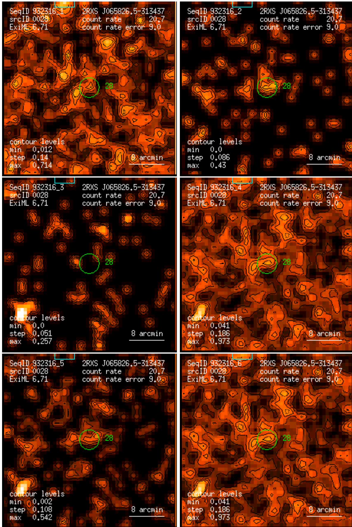
Figure 28: RASS 932316: detection 0028: band rate images, Gaussian filter: (1) PSPC channels 11 – 41, (2) 52 – 90, (3) 91 – 201, (4) 11 – 235, (5) 52 – 201, (6) 11 – 201. Broad band rates in counts/ks. Band rate contour levels in counts/ks/arcmin 2 .
