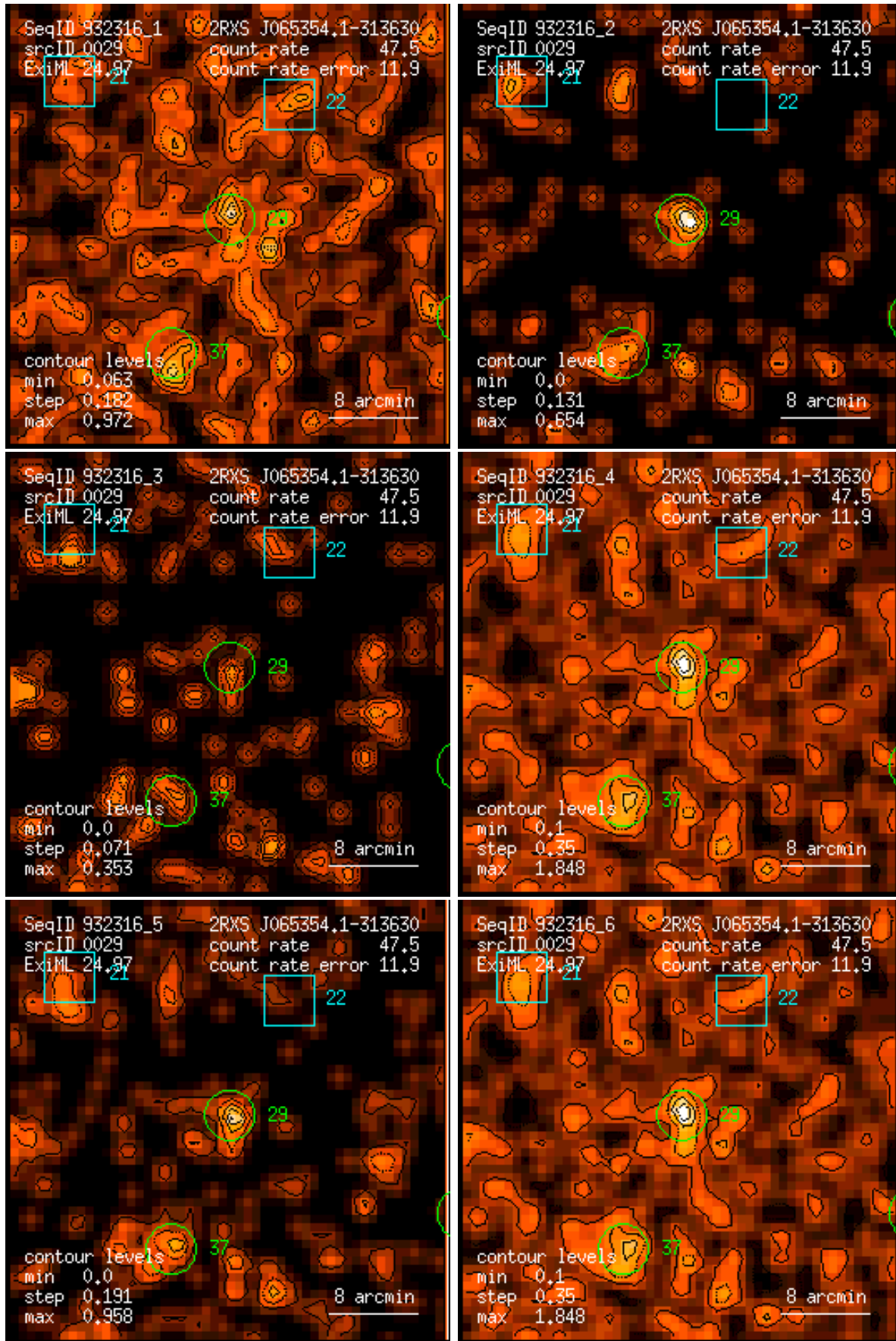
Figure 29: RASS 932316: detection 0029: band rate images, Gaussian filter: (1) PSPC channels 11 – 41, (2) 52 – 90, (3) 91 – 201, (4) 11 – 235, (5) 52 – 201, (6) 11 – 201. Broad band rates in counts/ks. Band rate contour levels in counts/ks/arcmin 2 .
