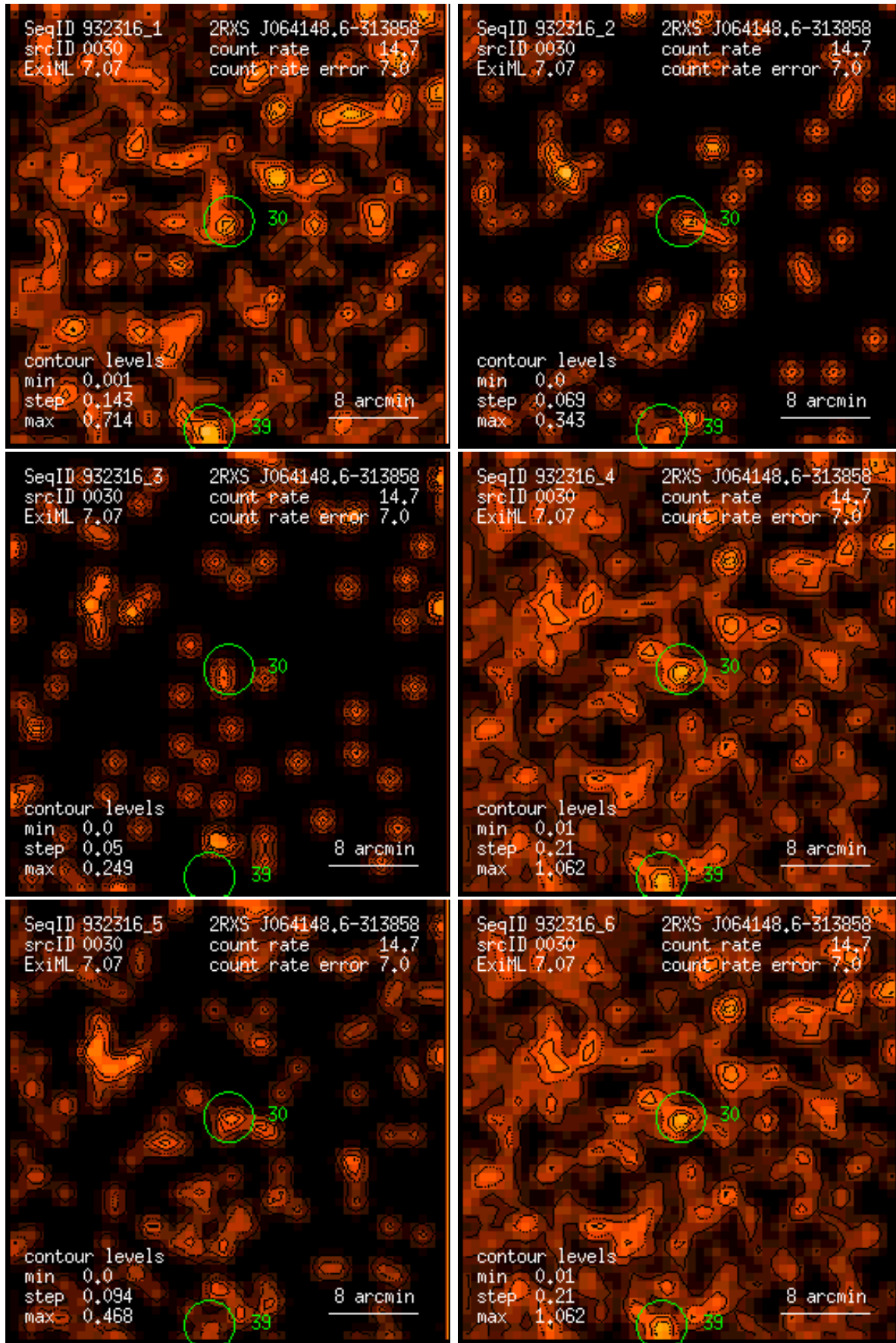
Figure 30: RASS 932316: detection 0030: band rate images, Gaussian filter: (1) PSPC channels 11 – 41, (2) 52 – 90, (3) 91 – 201, (4) 11 – 235, (5) 52 – 201, (6) 11 – 201. Broad band rates in counts/ks. Band rate contour levels in counts/ks/arcmin 2 .
