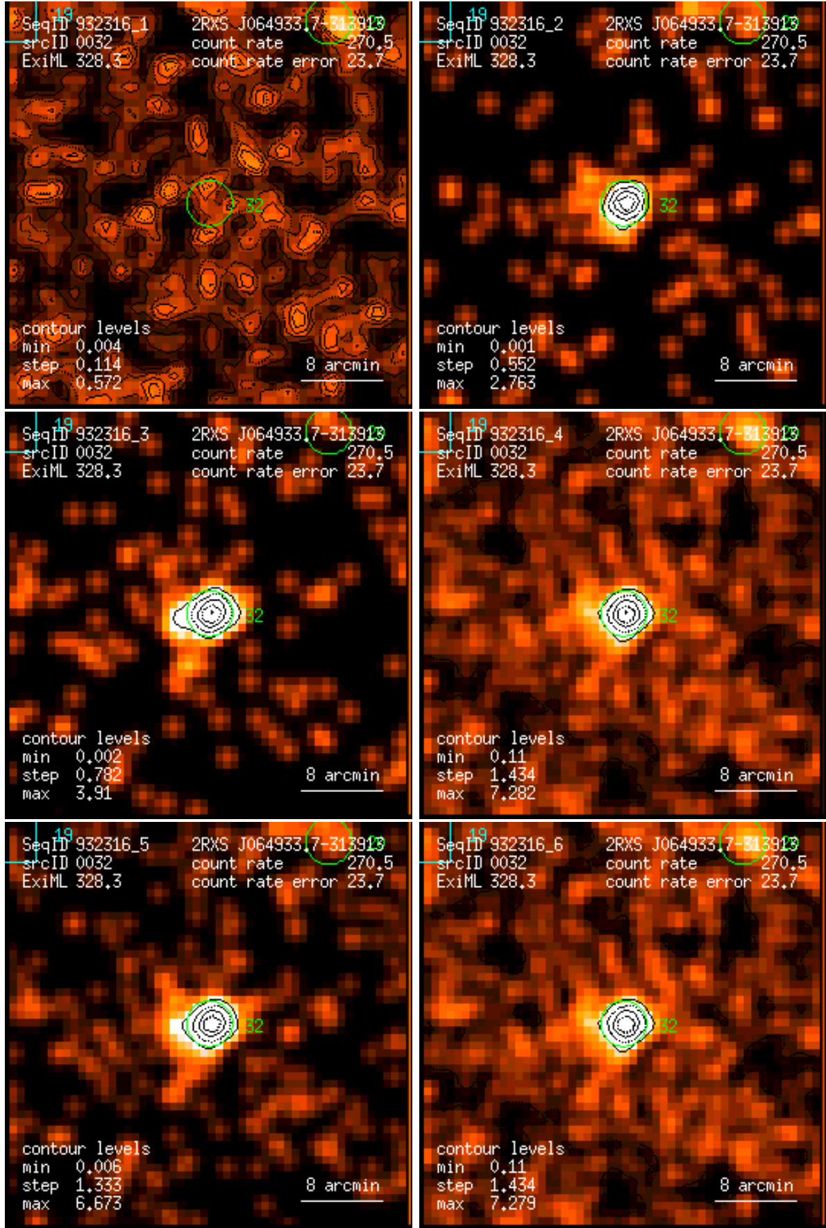
Figure 32: RASS 932316: detection 0032: band rate images, Gaussian filter: (1) PSPC channels 11 – 41, (2) 52 – 90, (3) 91 – 201, (4) 11 – 235, (5) 52 – 201, (6) 11 – 201. Broad band rates in counts/ks. Band rate contour levels in counts/ks/arcmin 2 .
