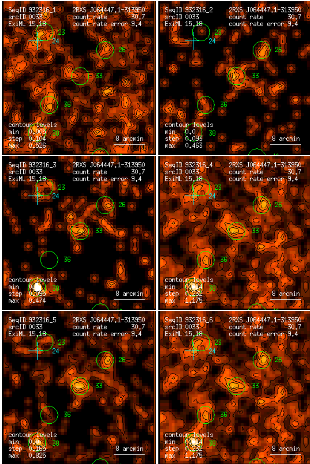
Figure 33: RASS 932316: detection 0033: band rate images, Gaussian filter: (1) PSPC channels 11 – 41, (2) 52 – 90, (3) 91 – 201, (4) 11 – 235, (5) 52 – 201, (6) 11 – 201. Broad band rates in counts/ks. Band rate contour levels in counts/ks/arcmin 2 .
