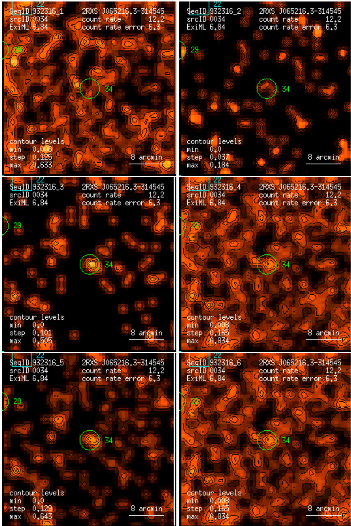
Figure 34: RASS 932316: detection 0034: band rate images, Gaussian filter: (1) PSPC channels 11 – 41, (2) 52 – 90, (3) 91 – 201, (4) 11 – 235, (5) 52 – 201, (6) 11 – 201. Broad band rates in counts/ks. Band rate contour levels in counts/ks/arcmin 2 .
