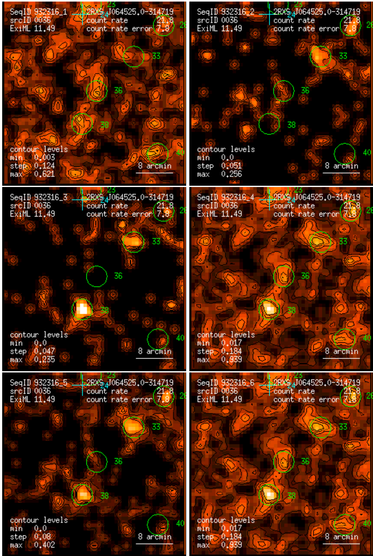
Figure 36: RASS 932316: detection 0036: band rate images, Gaussian filter: (1) PSPC channels 11 – 41, (2) 52 – 90, (3) 91 – 201, (4) 11 – 235, (5) 52 – 201, (6) 11 – 201. Broad band rates in counts/ks. Band rate contour levels in counts/ks/arcmin 2 .
