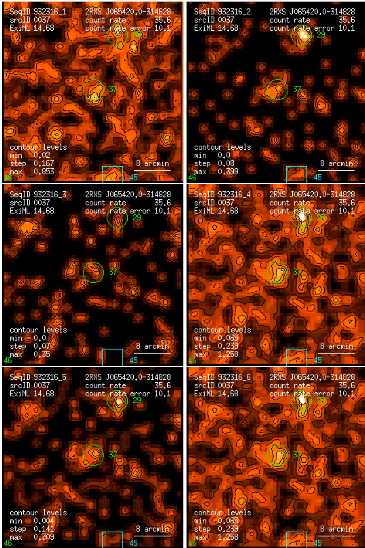
Figure 37: RASS 932316: detection 0037: band rate images, Gaussian filter: (1) PSPC channels 11 – 41, (2) 52 – 90, (3) 91 – 201, (4) 11 – 235, (5) 52 – 201, (6) 11 – 201. Broad band rates in counts/ks. Band rate contour levels in counts/ks/arcmin 2 .
