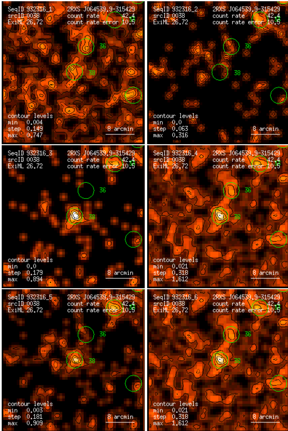
Figure 38: RASS 932316: detection 0038: band rate images, Gaussian filter: (1) PSPC channels 11 – 41, (2) 52 – 90, (3) 91 – 201, (4) 11 – 235, (5) 52 – 201, (6) 11 – 201. Broad band rates in counts/ks. Band rate contour levels in counts/ks/arcmin 2 .
