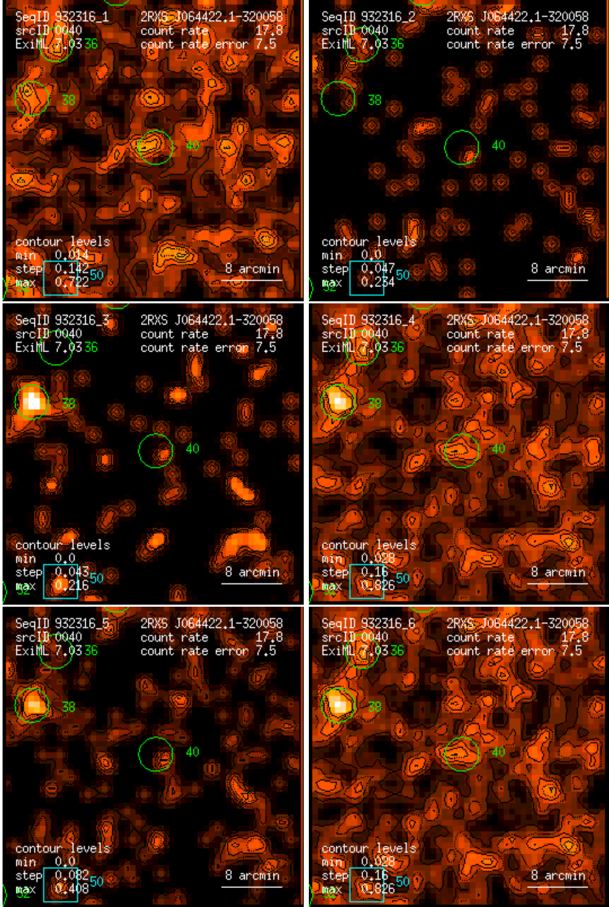
Figure 40: RASS 932316: detection 0040: band rate images, Gaussian filter: (1) PSPC channels 11 – 41, (2) 52 – 90, (3) 91 – 201, (4) 11 – 235, (5) 52 – 201, (6) 11 – 201. Broad band rates in counts/ks. Band rate contour levels in counts/ks/arcmin 2 .
