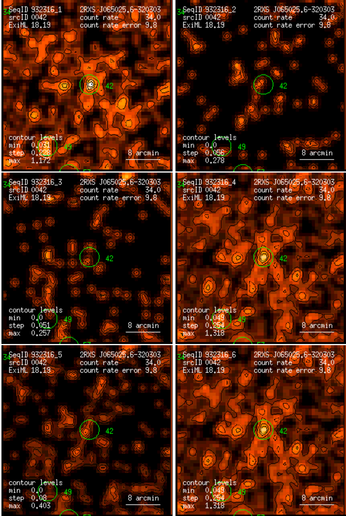
Figure 42: RASS 932316: detection 0042: band rate images, Gaussian filter: (1) PSPC channels 11 – 41, (2) 52 – 90, (3) 91 – 201, (4) 11 – 235, (5) 52 – 201, (6) 11 – 201. Broad band rates in counts/ks. Band rate contour levels in counts/ks/arcmin 2 .
