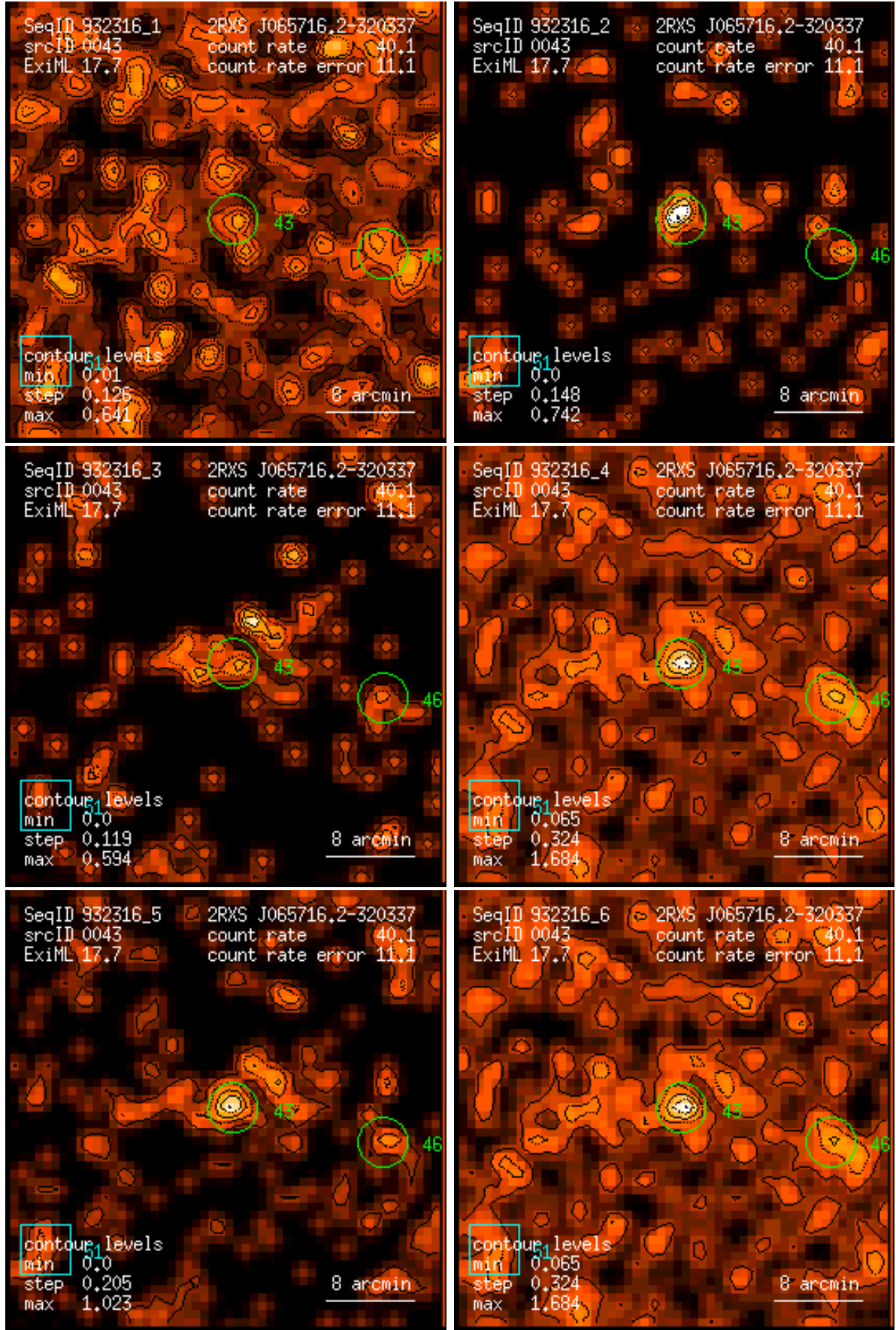
Figure 43: RASS 932316: detection 0043: band rate images, Gaussian filter: (1) PSPC channels 11 – 41, (2) 52 – 90, (3) 91 – 201, (4) 11 – 235, (5) 52 – 201, (6) 11 – 201. Broad band rates in counts/ks. Band rate contour levels in counts/ks/arcmin 2 .
