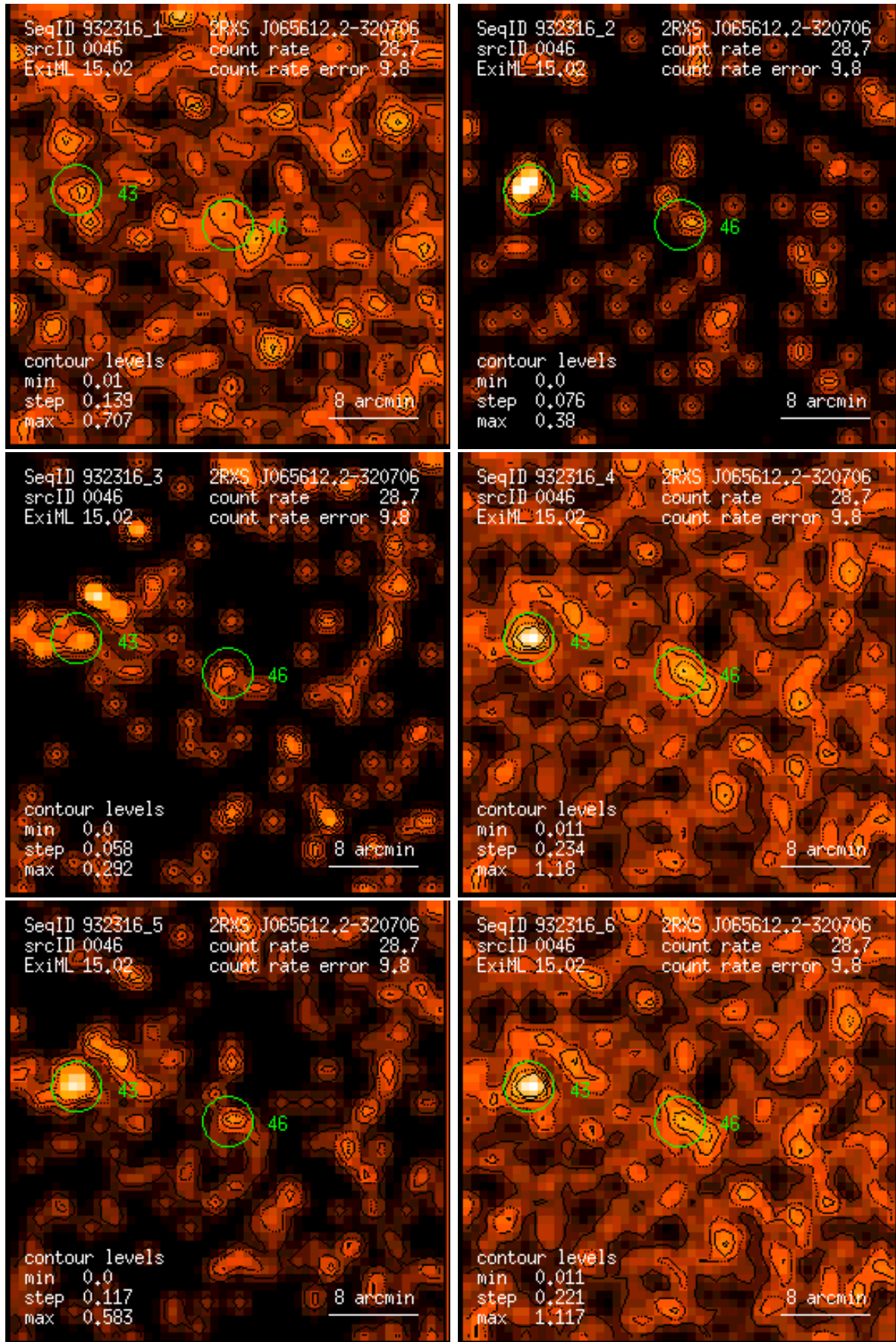
Figure 46: RASS 932316: detection 0046: band rate images, Gaussian filter: (1) PSPC channels 11 – 41, (2) 52 – 90, (3) 91 – 201, (4) 11 – 235, (5) 52 – 201, (6) 11 – 201. Broad band rates in counts/ks. Band rate contour levels in counts/ks/arcmin 2 .
