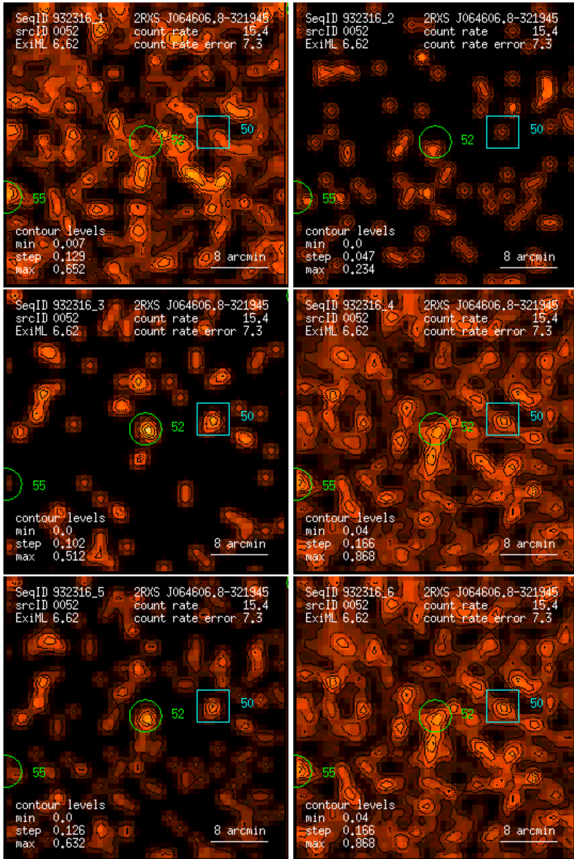
Figure 52: RASS 932316: detection 0052: band rate images, Gaussian filter: (1) PSPC channels 11 – 41, (2) 52 – 90, (3) 91 – 201, (4) 11 – 235, (5) 52 – 201, (6) 11 – 201. Broad band rates in counts/ks. Band rate contour levels in counts/ks/arcmin 2 .
