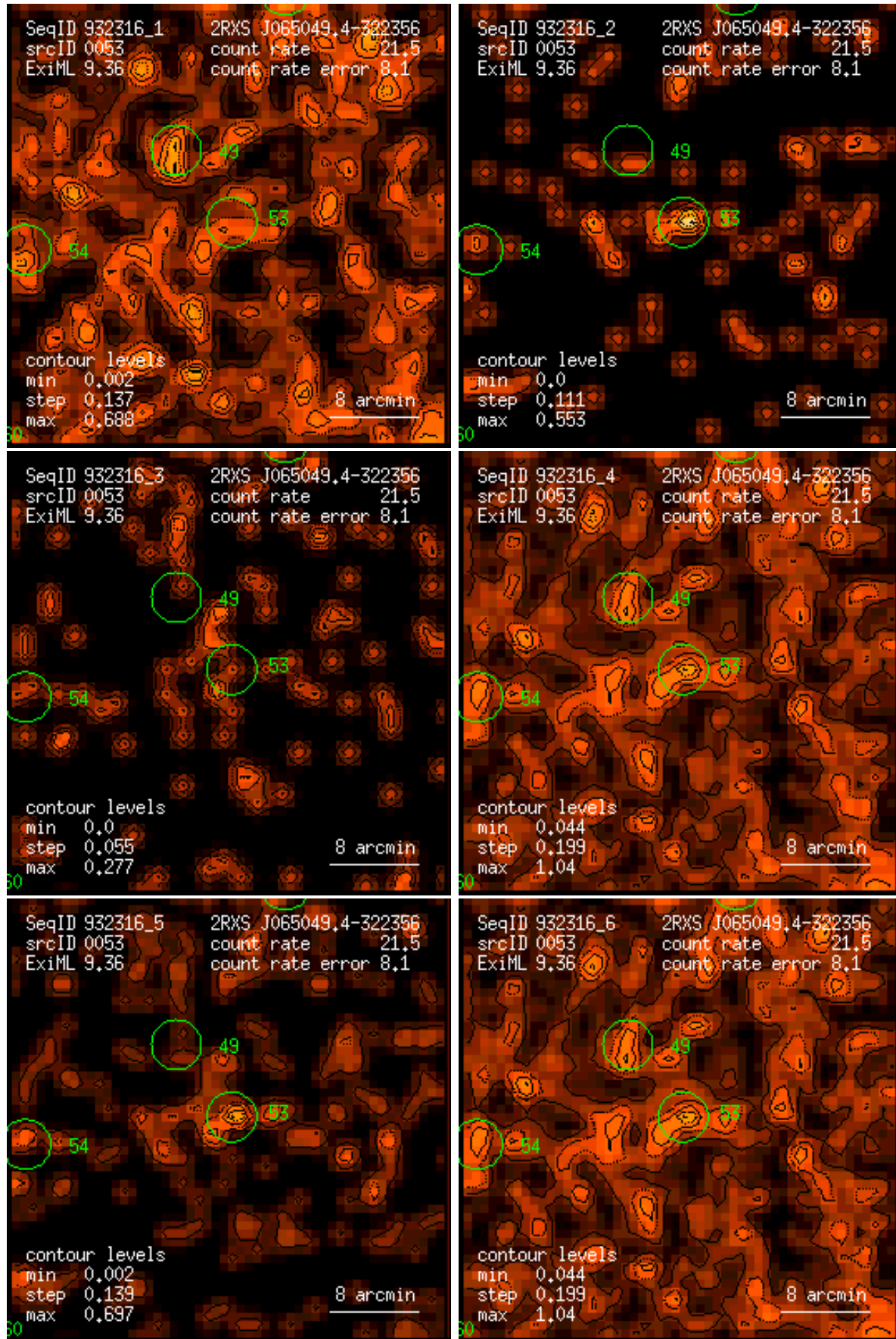
Figure 53: RASS 932316: detection 0053: band rate images, Gaussian filter: (1) PSPC channels 11 – 41, (2) 52 – 90, (3) 91 – 201, (4) 11 – 235, (5) 52 – 201, (6) 11 – 201. Broad band rates in counts/ks. Band rate contour levels in counts/ks/arcmin 2 .
