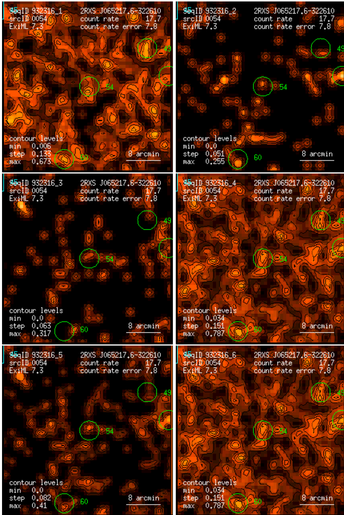
Figure 54: RASS 932316: detection 0054: band rate images, Gaussian filter: (1) PSPC channels 11 – 41, (2) 52 – 90, (3) 91 – 201, (4) 11 – 235, (5) 52 – 201, (6) 11 – 201. Broad band rates in counts/ks. Band rate contour levels in counts/ks/arcmin 2 .
