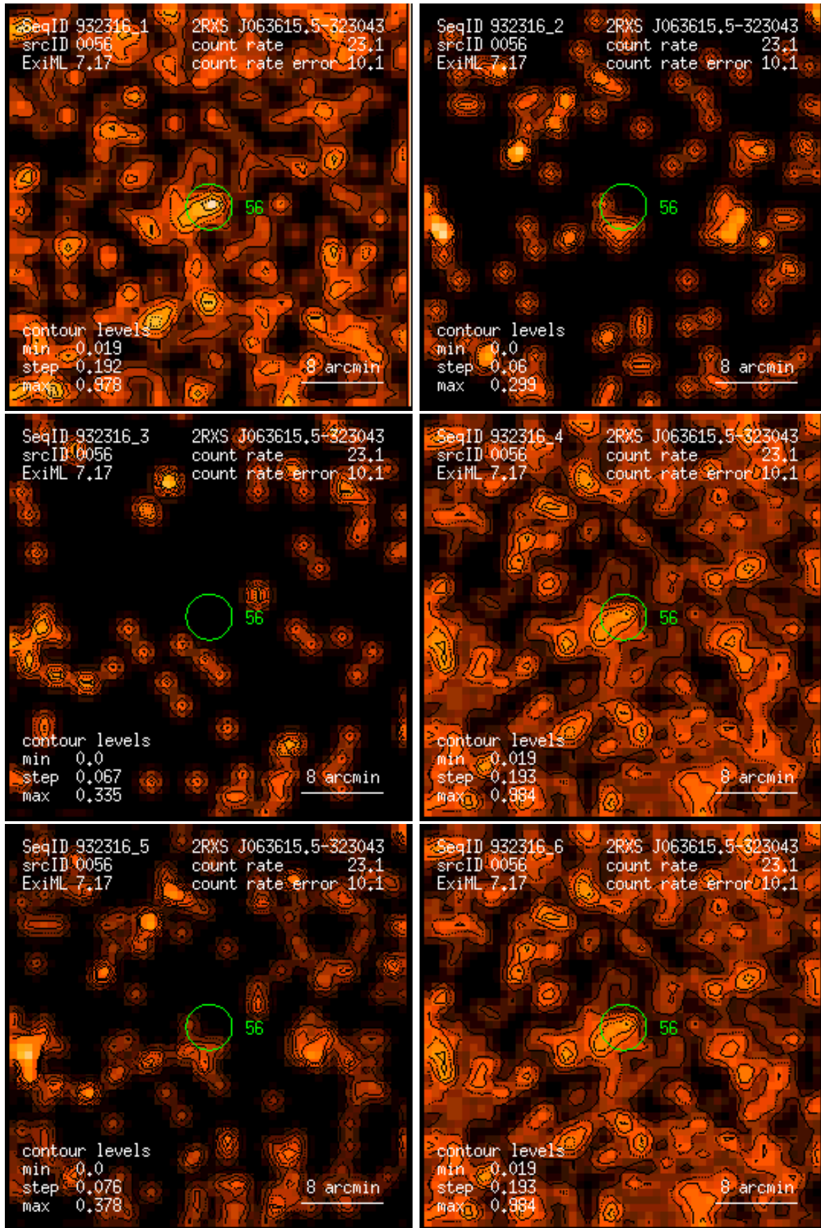
Figure 56: RASS 932316: detection 0056: band rate images, Gaussian filter: (1) PSPC channels 11 – 41, (2) 52 – 90, (3) 91 – 201, (4) 11 – 235, (5) 52 – 201, (6) 11 – 201. Broad band rates in counts/ks. Band rate contour levels in counts/ks/arcmin 2 .
