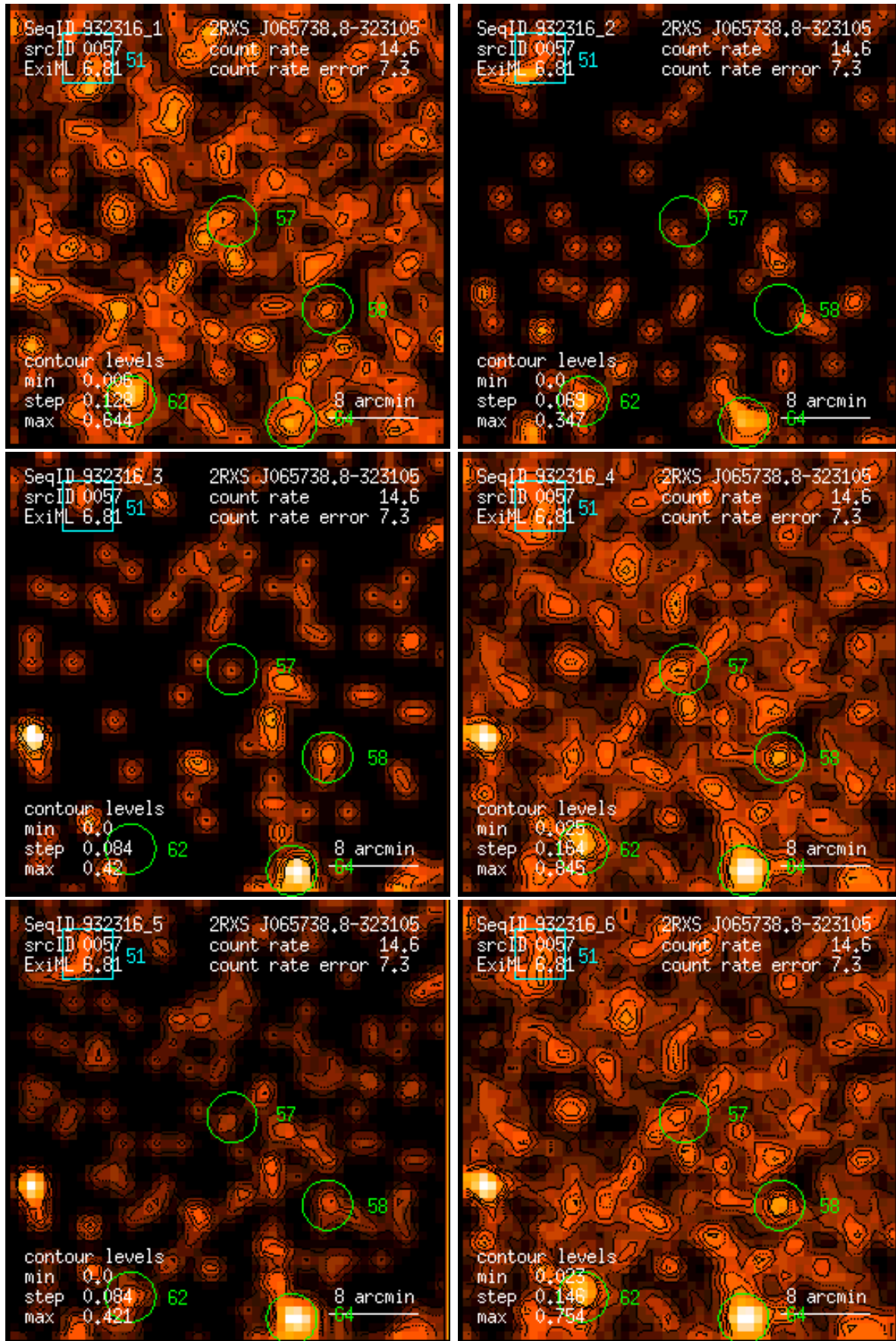
Figure 57: RASS 932316: detection 0057: band rate images, Gaussian filter: (1) PSPC channels 11 – 41, (2) 52 – 90, (3) 91 – 201, (4) 11 – 235, (5) 52 – 201, (6) 11 – 201. Broad band rates in counts/ks. Band rate contour levels in counts/ks/arcmin 2 .
