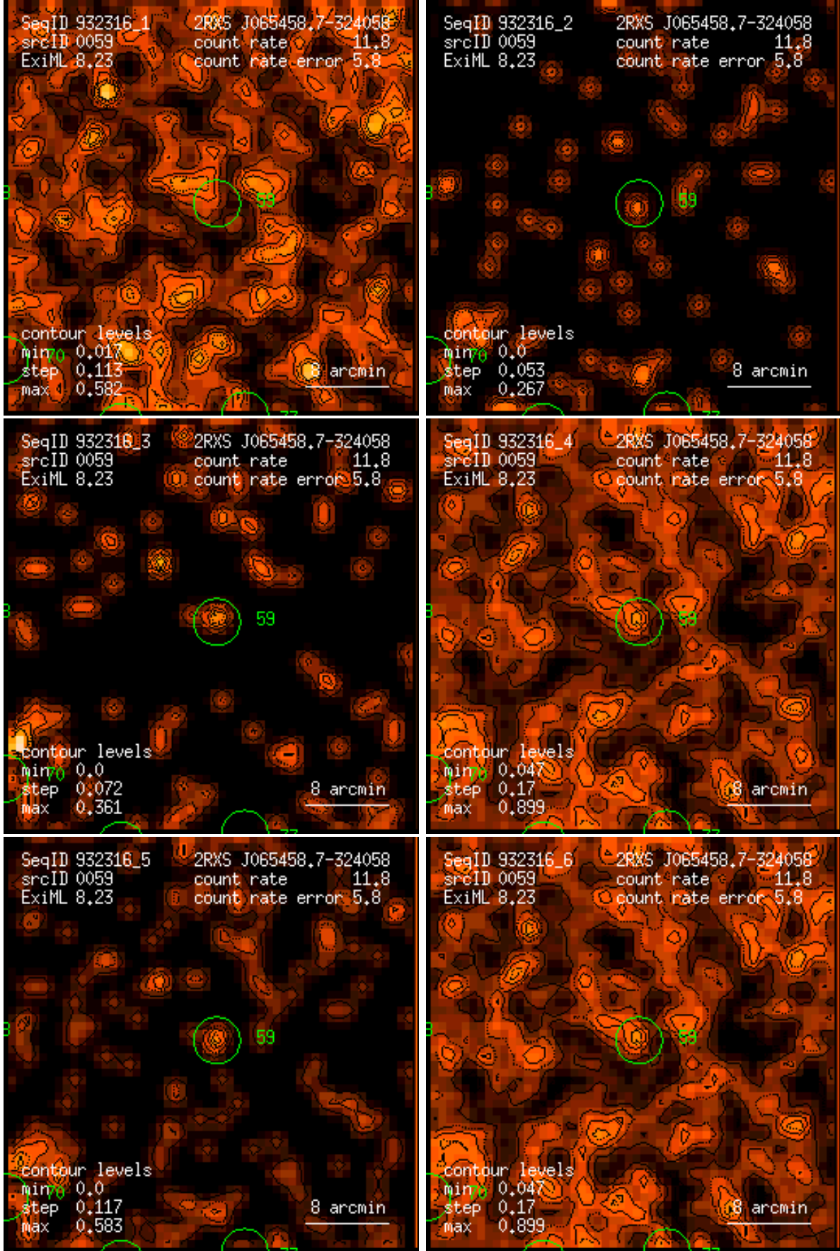
Figure 59: RASS 932316: detection 0059: band rate images, Gaussian filter: (1) PSPC channels 11 – 41, (2) 52 – 90, (3) 91 – 201, (4) 11 – 235, (5) 52 – 201, (6) 11 – 201. Broad band rates in counts/ks. Band rate contour levels in counts/ks/arcmin 2 .
