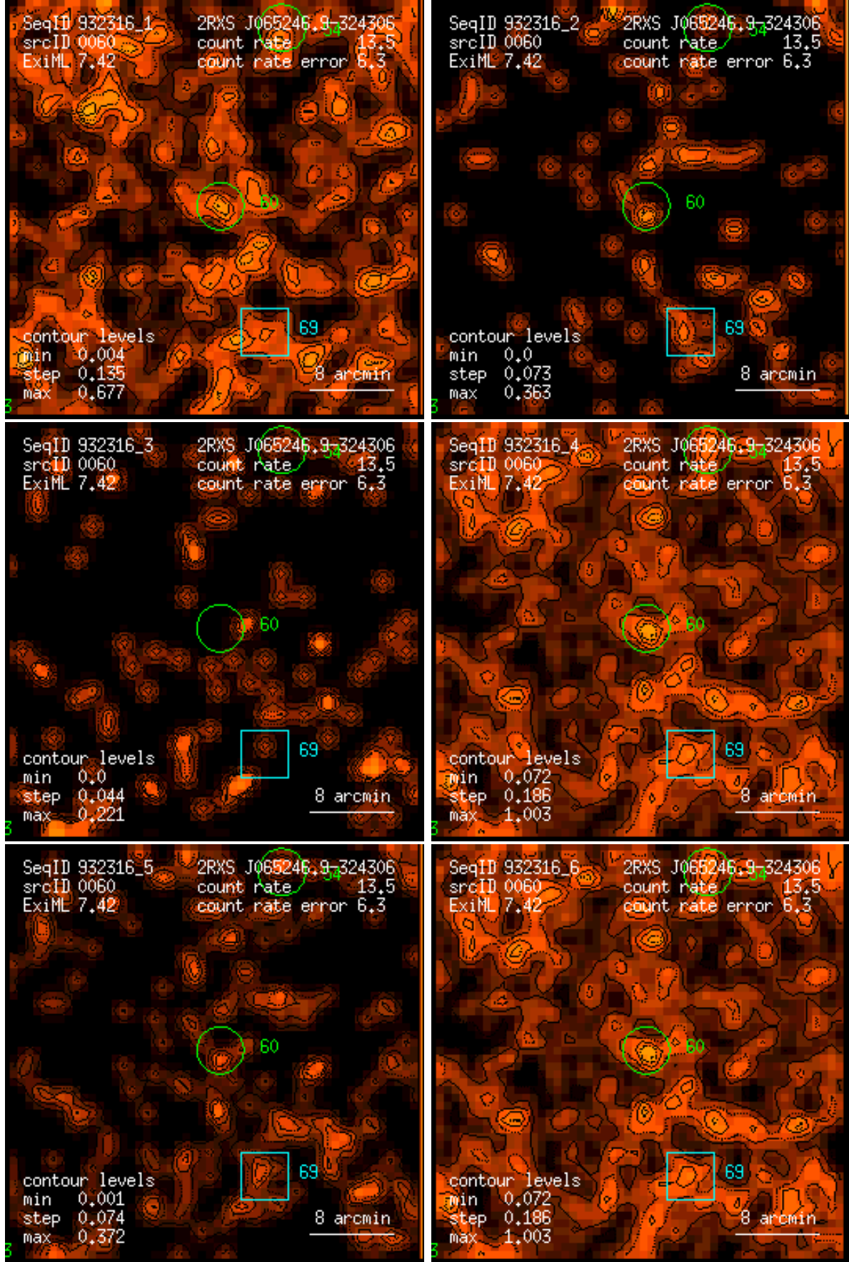
Figure 60: RASS 932316: detection 0060: band rate images, Gaussian filter: (1) PSPC channels 11 – 41, (2) 52 – 90, (3) 91 – 201, (4) 11 – 235, (5) 52 – 201, (6) 11 – 201. Broad band rates in counts/ks. Band rate contour levels in counts/ks/arcmin 2 .
