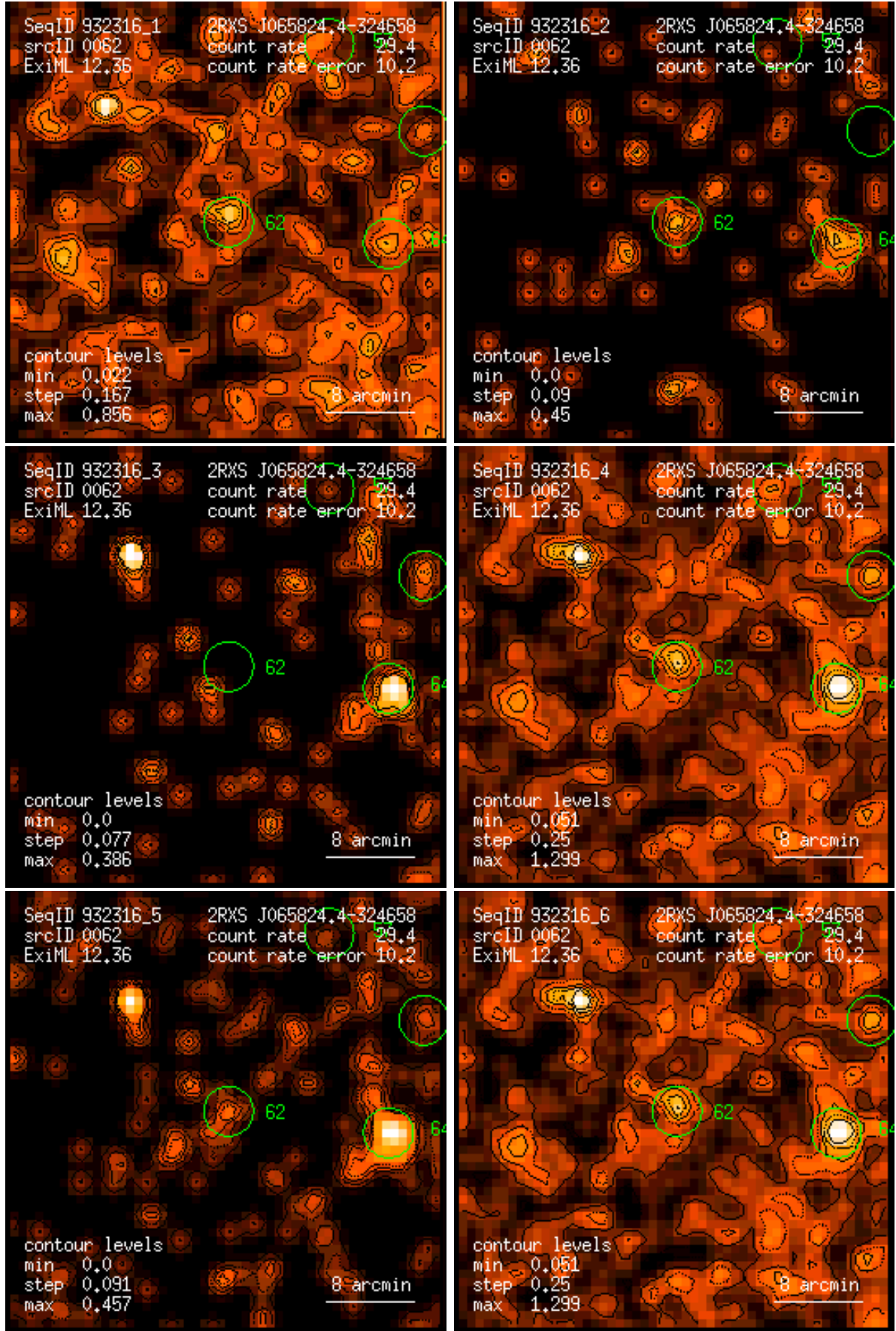
Figure 62: RASS 932316: detection 0062: band rate images, Gaussian filter: (1) PSPC channels 11 – 41, (2) 52 – 90, (3) 91 – 201, (4) 11 – 235, (5) 52 – 201, (6) 11 – 201. Broad band rates in counts/ks. Band rate contour levels in counts/ks/arcmin 2 .
