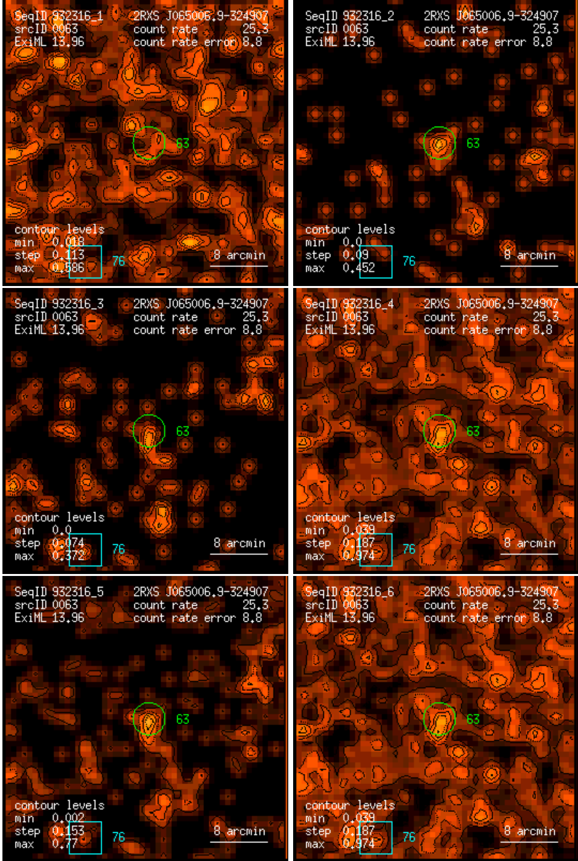
Figure 63: RASS 932316: detection 0063: band rate images, Gaussian filter: (1) PSPC channels 11 – 41, (2) 52 – 90, (3) 91 – 201, (4) 11 – 235, (5) 52 – 201, (6) 11 – 201. Broad band rates in counts/ks. Band rate contour levels in counts/ks/arcmin 2 .
