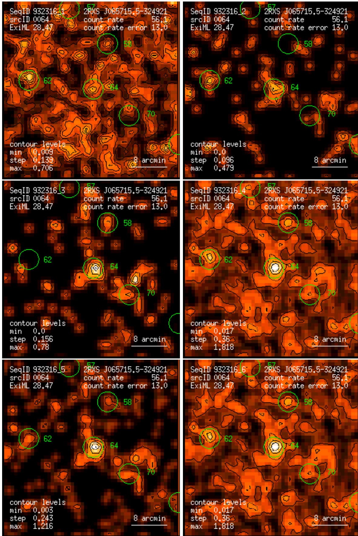
Figure 64: RASS 932316: detection 0064: band rate images, Gaussian filter: (1) PSPC channels 11 – 41, (2) 52 – 90, (3) 91 – 201, (4) 11 – 235, (5) 52 – 201, (6) 11 – 201. Broad band rates in counts/ks. Band rate contour levels in counts/ks/arcmin 2 .
