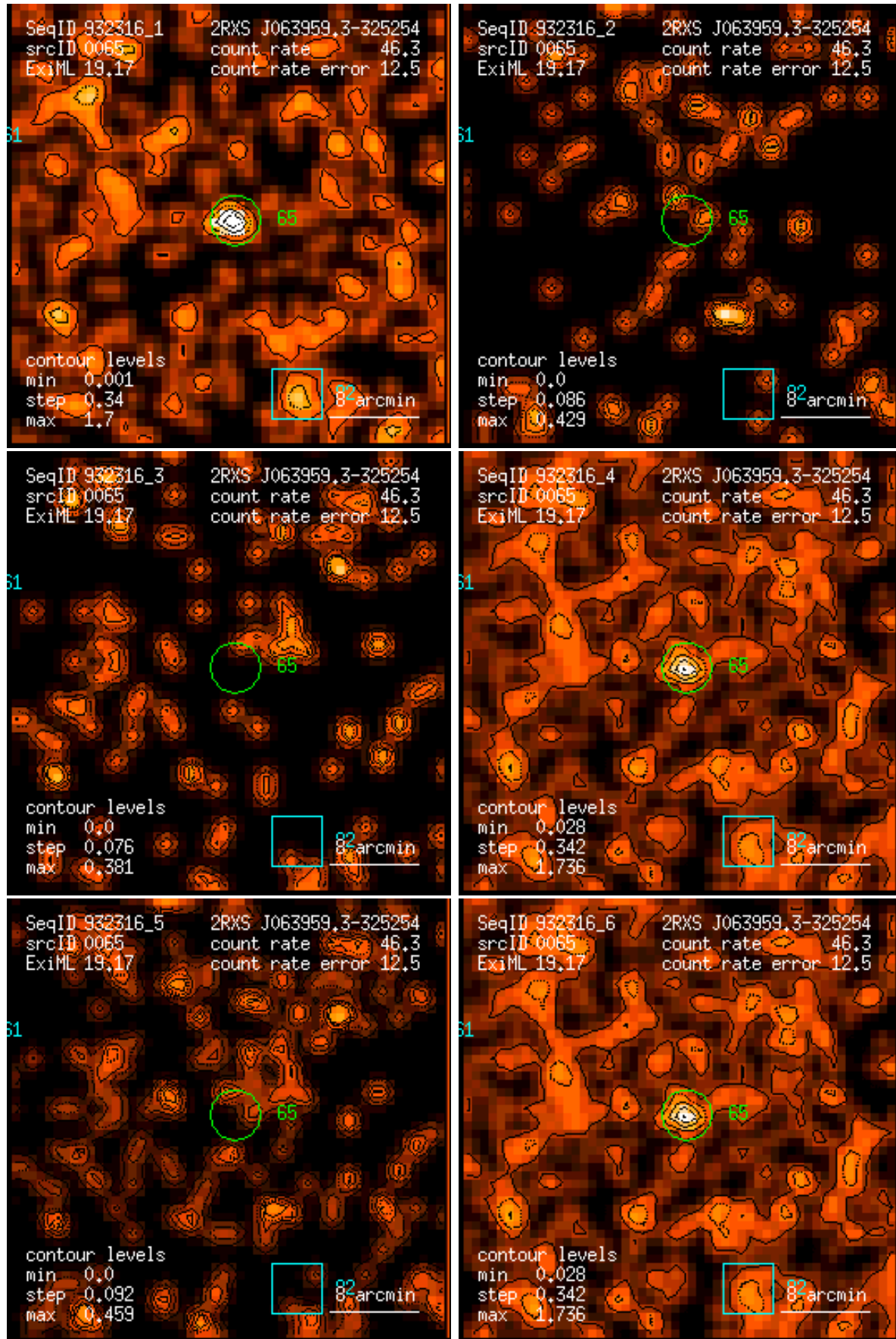
Figure 65: RASS 932316: detection 0065: band rate images, Gaussian filter: (1) PSPC channels 11 – 41, (2) 52 – 90, (3) 91 – 201, (4) 11 – 235, (5) 52 – 201, (6) 11 – 201. Broad band rates in counts/ks. Band rate contour levels in counts/ks/arcmin 2 .
