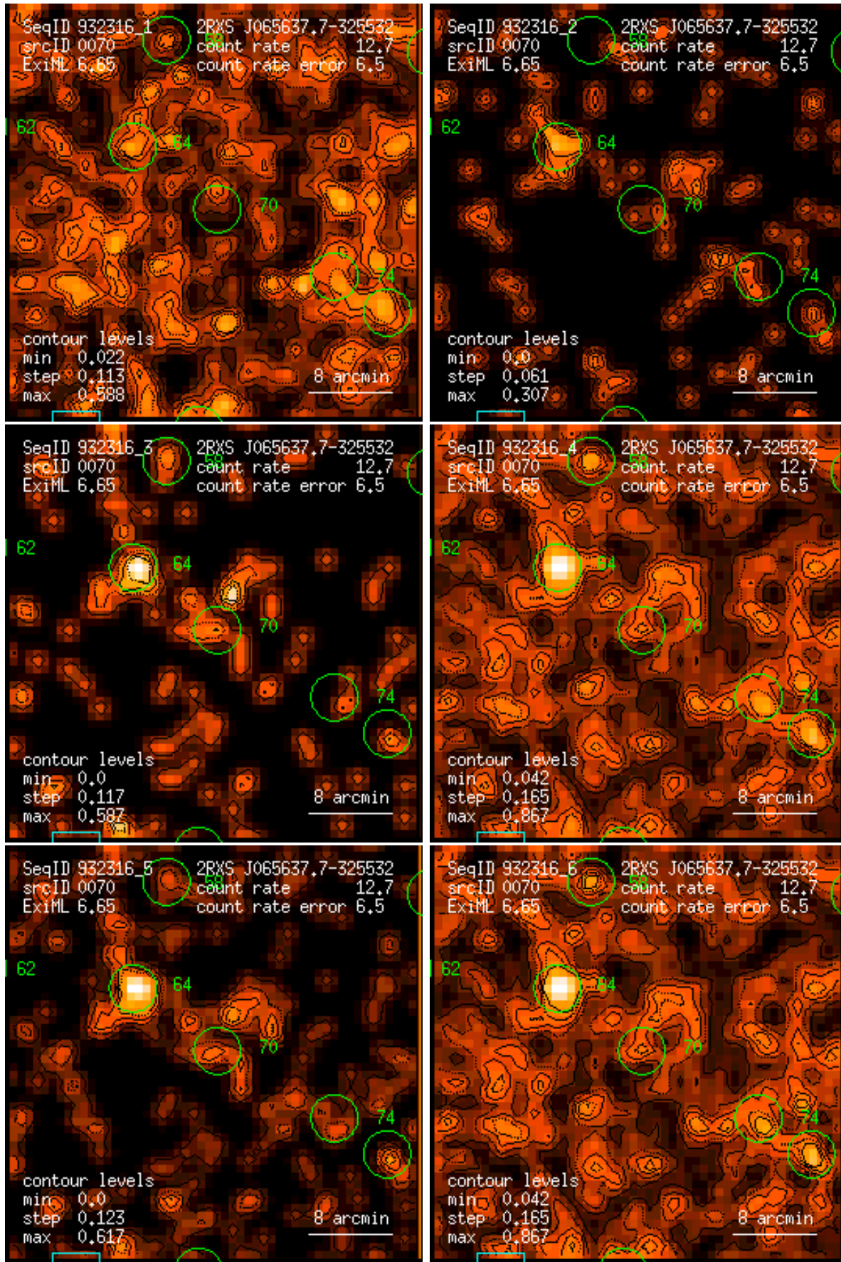
Figure 70: RASS 932316: detection 0070: band rate images, Gaussian filter: (1) PSPC channels 11 – 41, (2) 52 – 90, (3) 91 – 201, (4) 11 – 235, (5) 52 – 201, (6) 11 – 201. Broad band rates in counts/ks. Band rate contour levels in counts/ks/arcmin 2 .
