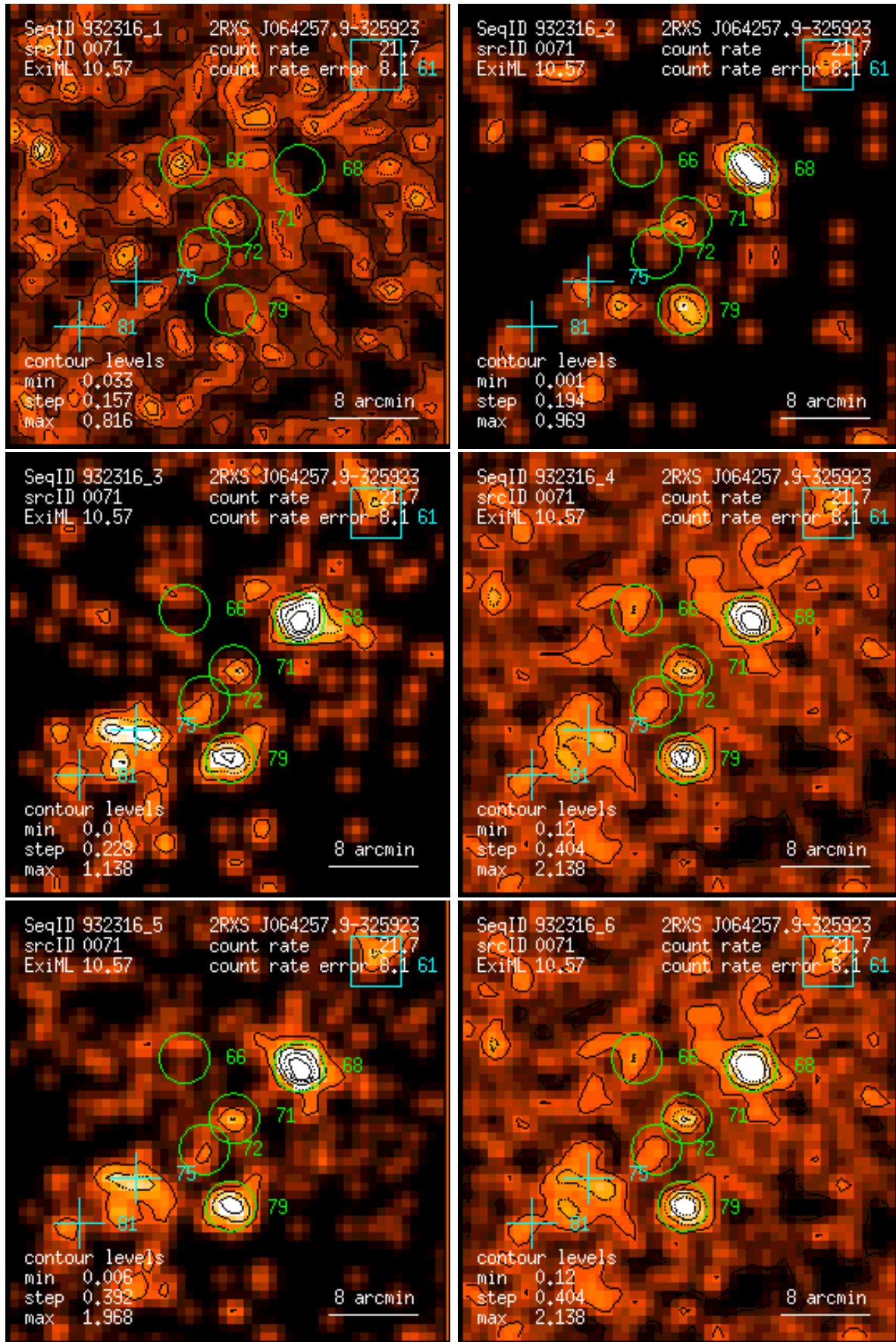
Figure 71: RASS 932316: detection 0071: band rate images, Gaussian filter: (1) PSPC channels 11 – 41, (2) 52 – 90, (3) 91 – 201, (4) 11 – 235, (5) 52 – 201, (6) 11 – 201. Broad band rates in counts/ks. Band rate contour levels in counts/ks/arcmin 2 .
