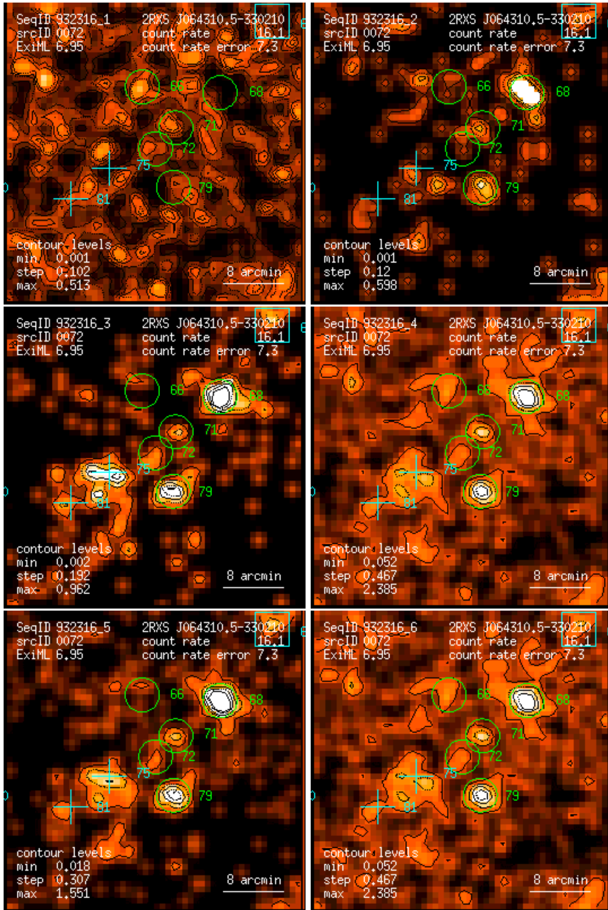
Figure 72: RASS 932316: detection 0072: band rate images, Gaussian filter: (1) PSPC channels 11 – 41, (2) 52 – 90, (3) 91 – 201, (4) 11 – 235, (5) 52 – 201, (6) 11 – 201. Broad band rates in counts/ks. Band rate contour levels in counts/ks/arcmin 2 .
