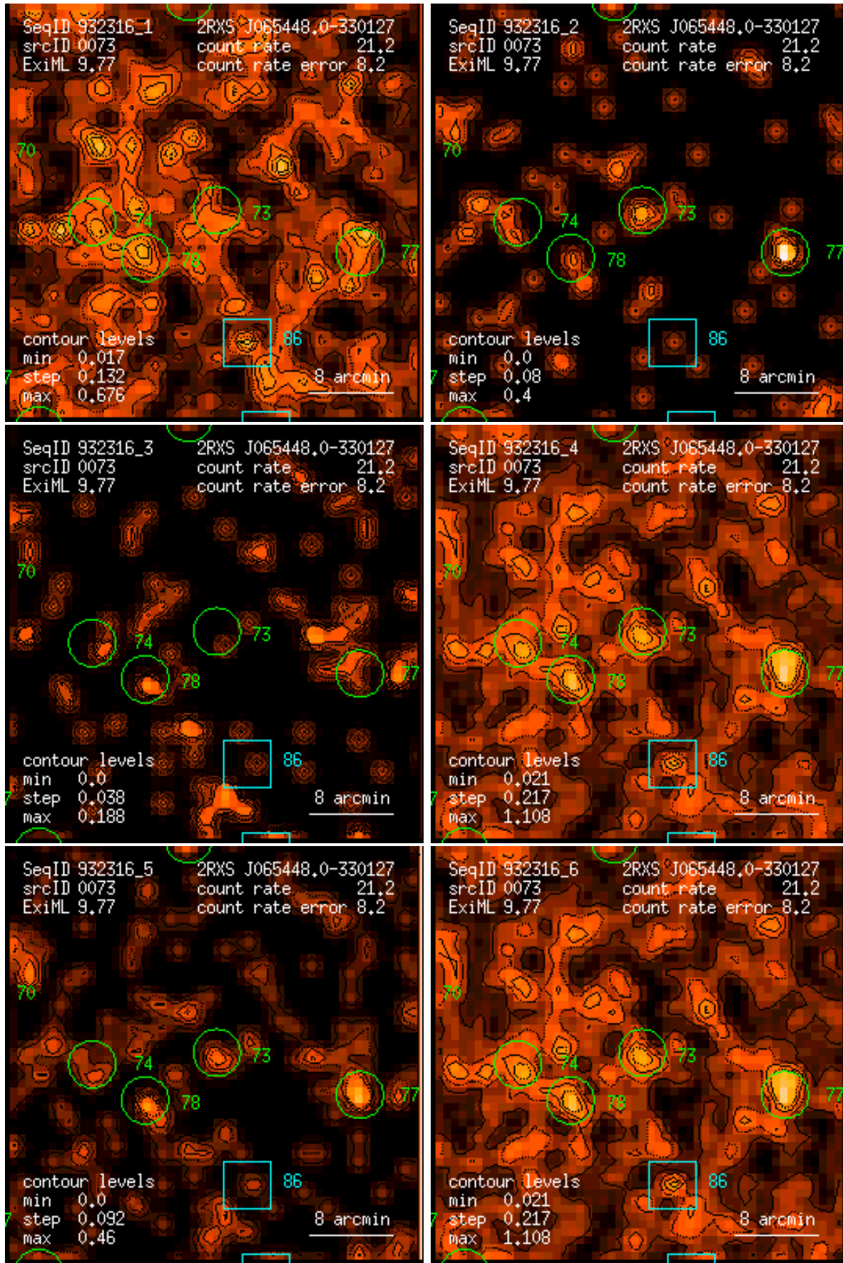
Figure 73: RASS 932316: detection 0073: band rate images, Gaussian filter: (1) PSPC channels 11 – 41, (2) 52 – 90, (3) 91 – 201, (4) 11 – 235, (5) 52 – 201, (6) 11 – 201. Broad band rates in counts/ks. Band rate contour levels in counts/ks/arcmin 2 .
