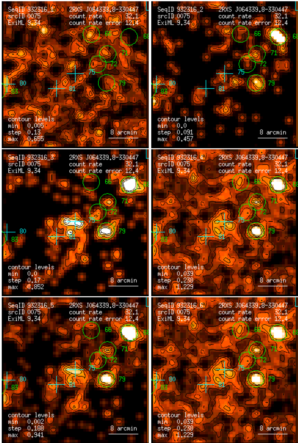
Figure 75: RASS 932316: detection 0075: band rate images, Gaussian filter: (1) PSPC channels 11 – 41, (2) 52 – 90, (3) 91 – 201, (4) 11 – 235, (5) 52 – 201, (6) 11 – 201. Broad band rates in counts/ks. Band rate contour levels in counts/ks/arcmin 2 .
