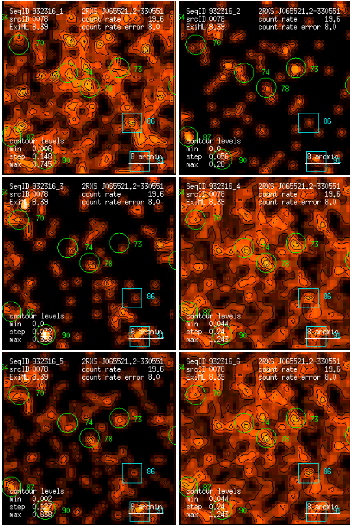
Figure 78: RASS 932316: detection 0078: band rate images, Gaussian filter: (1) PSPC channels 11 – 41, (2) 52 – 90, (3) 91 – 201, (4) 11 – 235, (5) 52 – 201, (6) 11 – 201. Broad band rates in counts/ks. Band rate contour levels in counts/ks/arcmin 2 .
